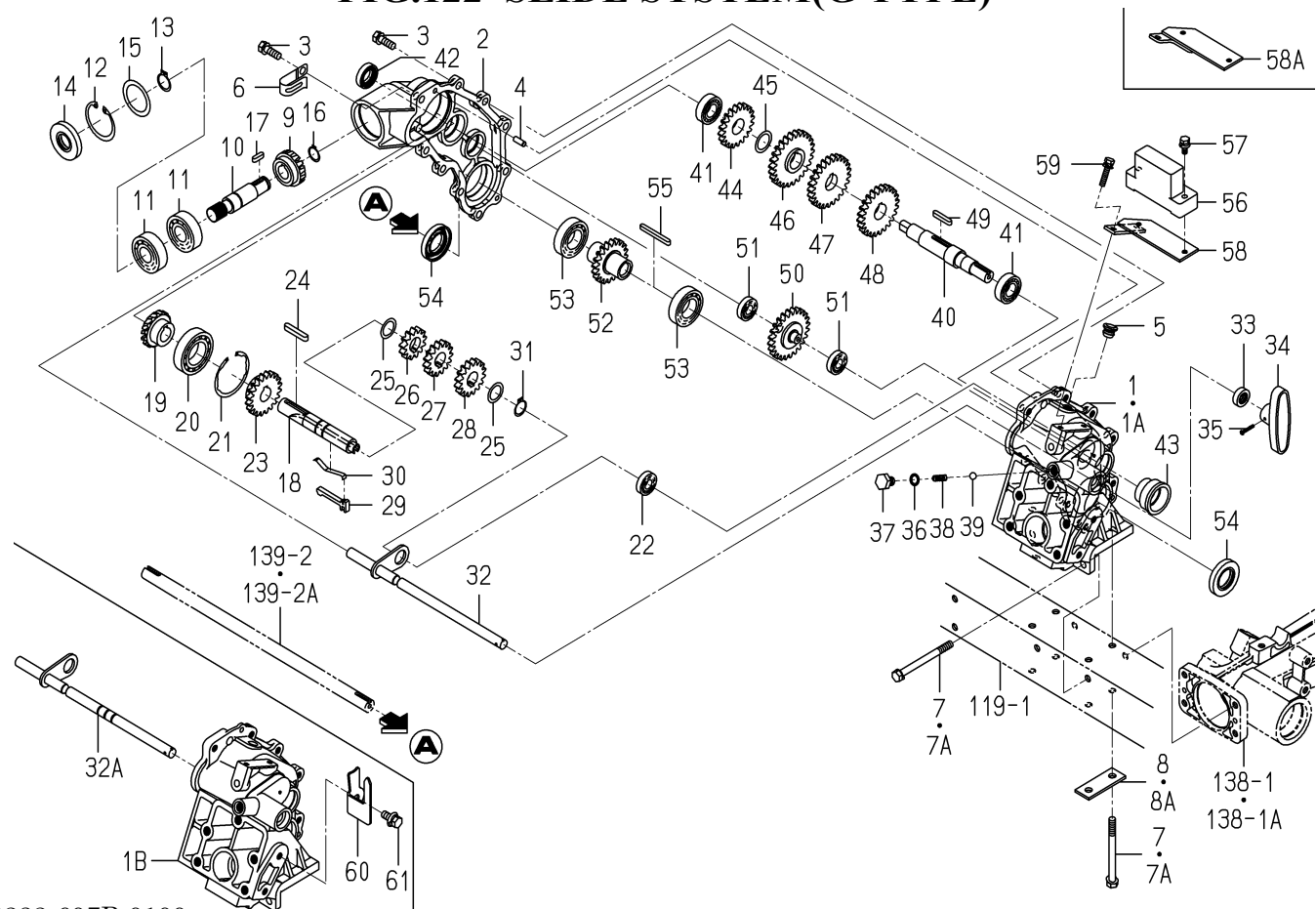
FIG.122 SLIDE SYSTEM(G TYPE)
