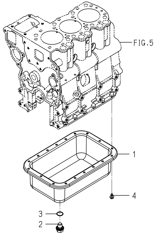
FIG. 7 OIL PAN
