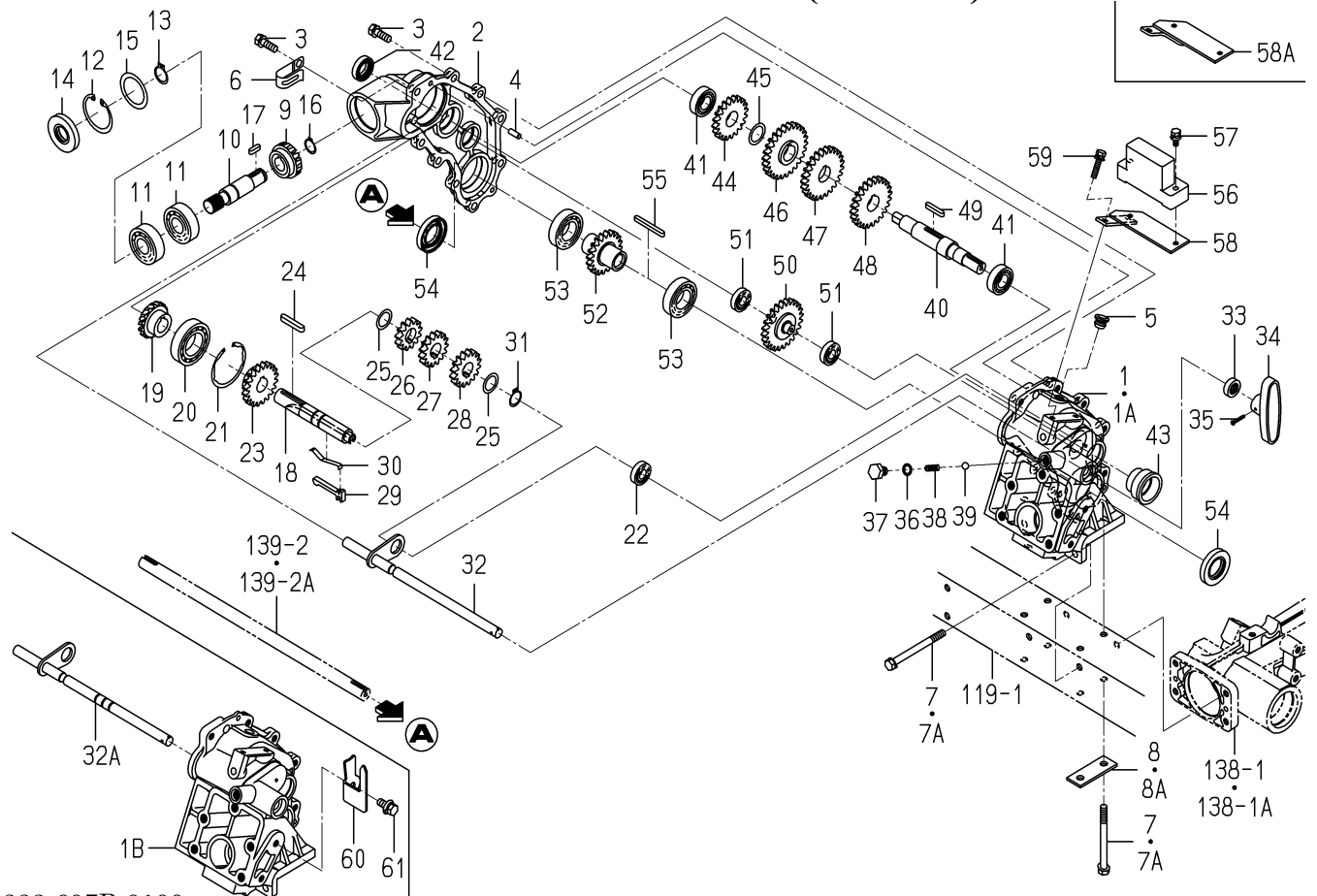
FIG.122 SLIDE SYSTEM(G TYPE)
