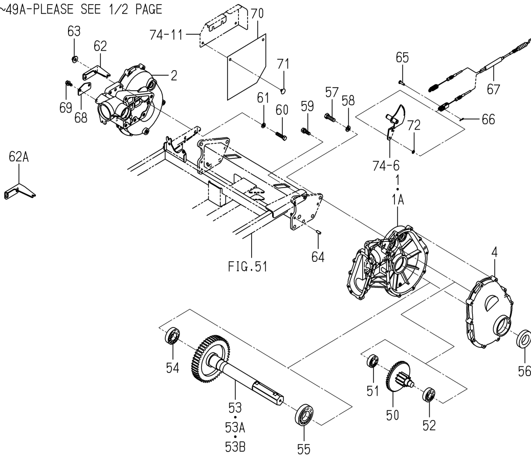
FIG. 57 CASE(REAR)SYSTEM(GF TYPE)(2/2)
