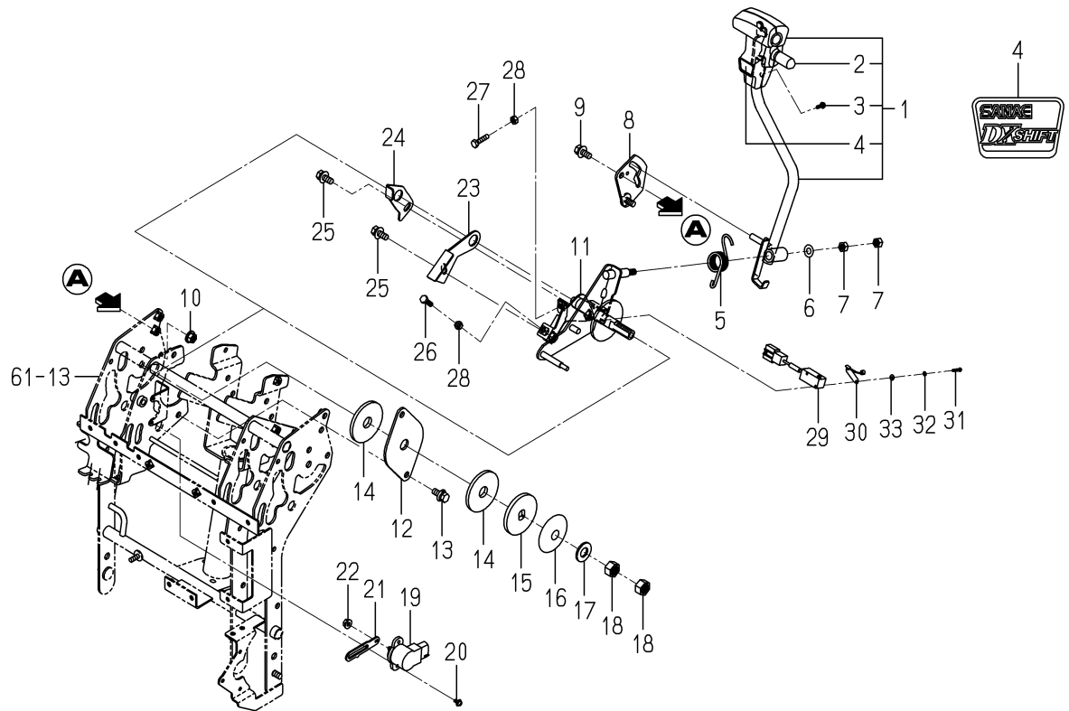
FIG. 14 LEVER(MAIN)SYSTEM(G TYPE)
