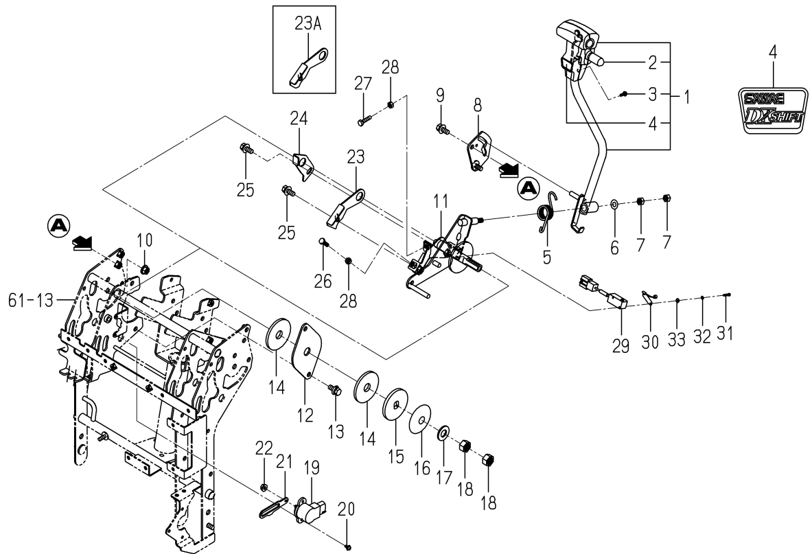
FIG. 15 LEVER(MAIN)SYSTEM(D TYPE)
