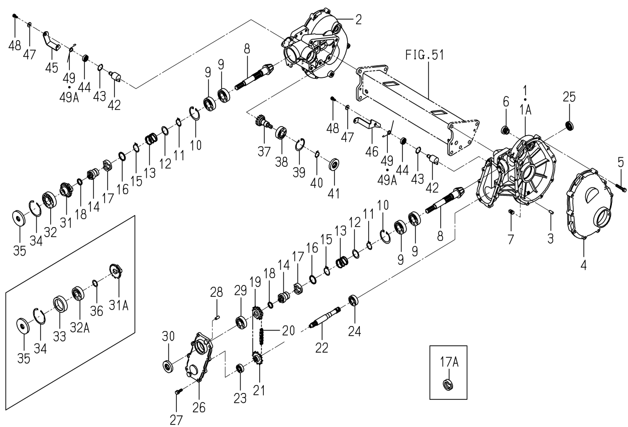
FIG. 57 CASE(REAR)SYSTEM(GF TYPE)(1/2)
