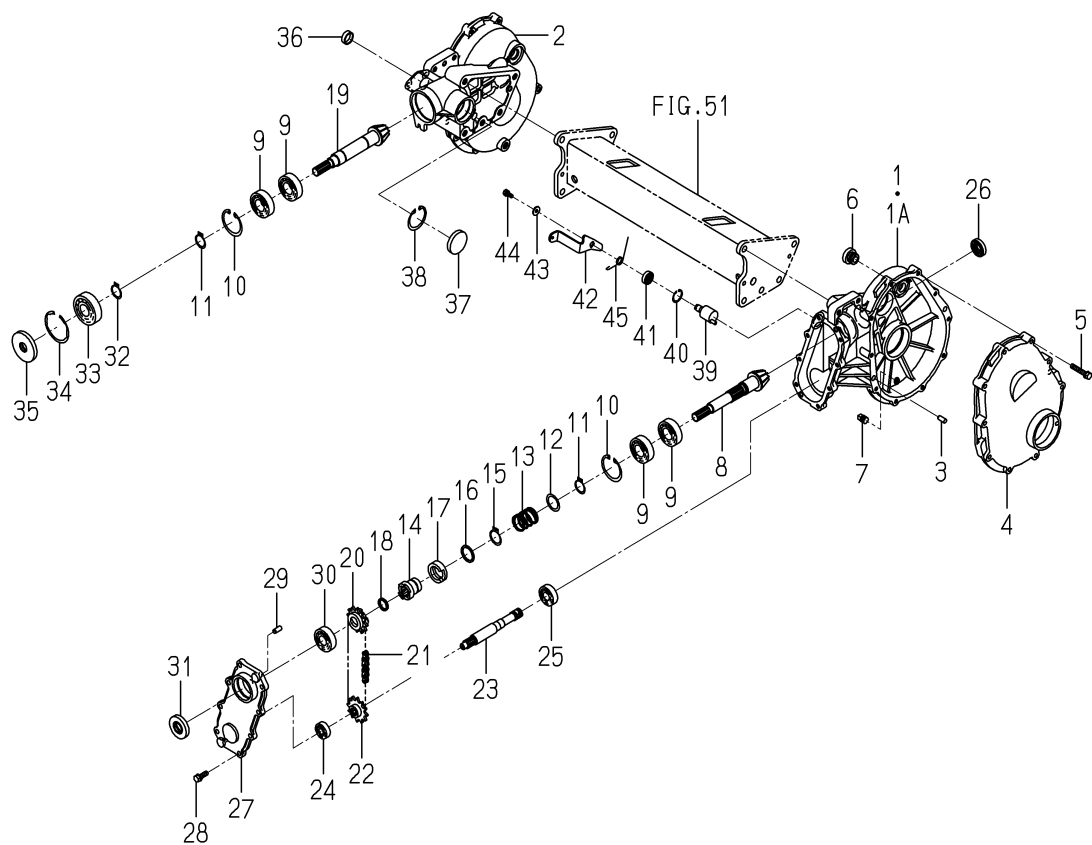
FIG. 59 CASE(REAR)SYSTEM(GF TYPE)(1/2)
