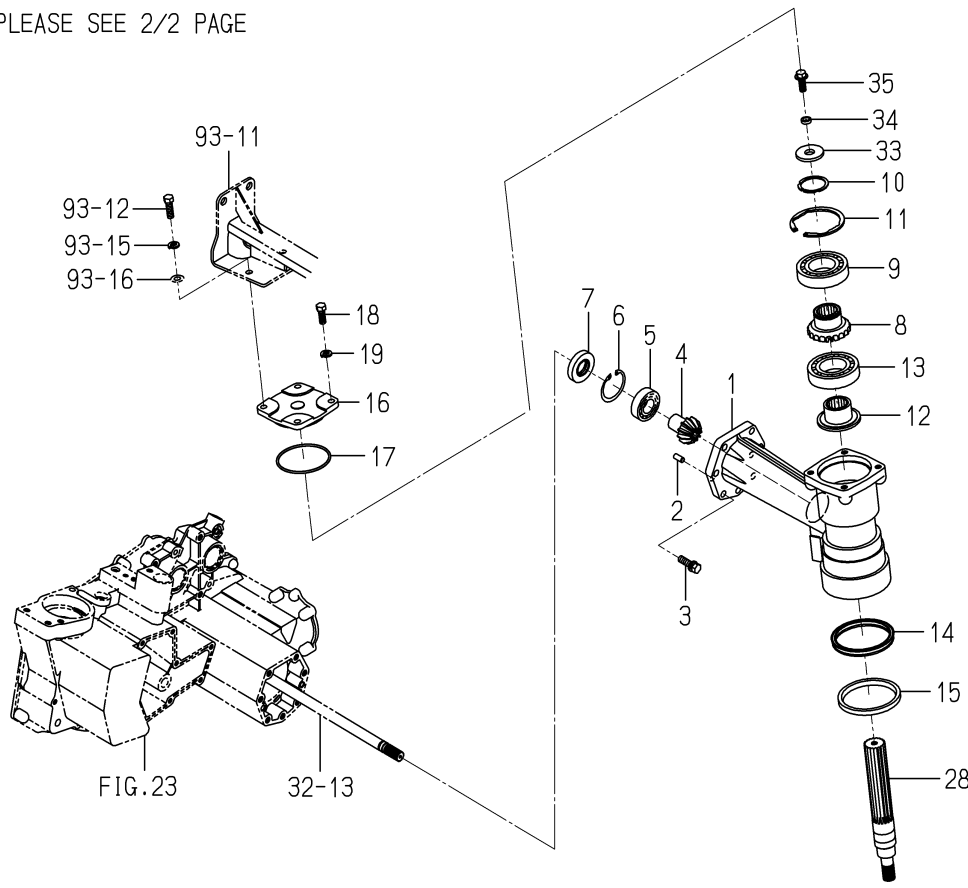
FIG. 46 CASE(GEAR/FINAL)SYSTEM(D TYPE)(1/2)
