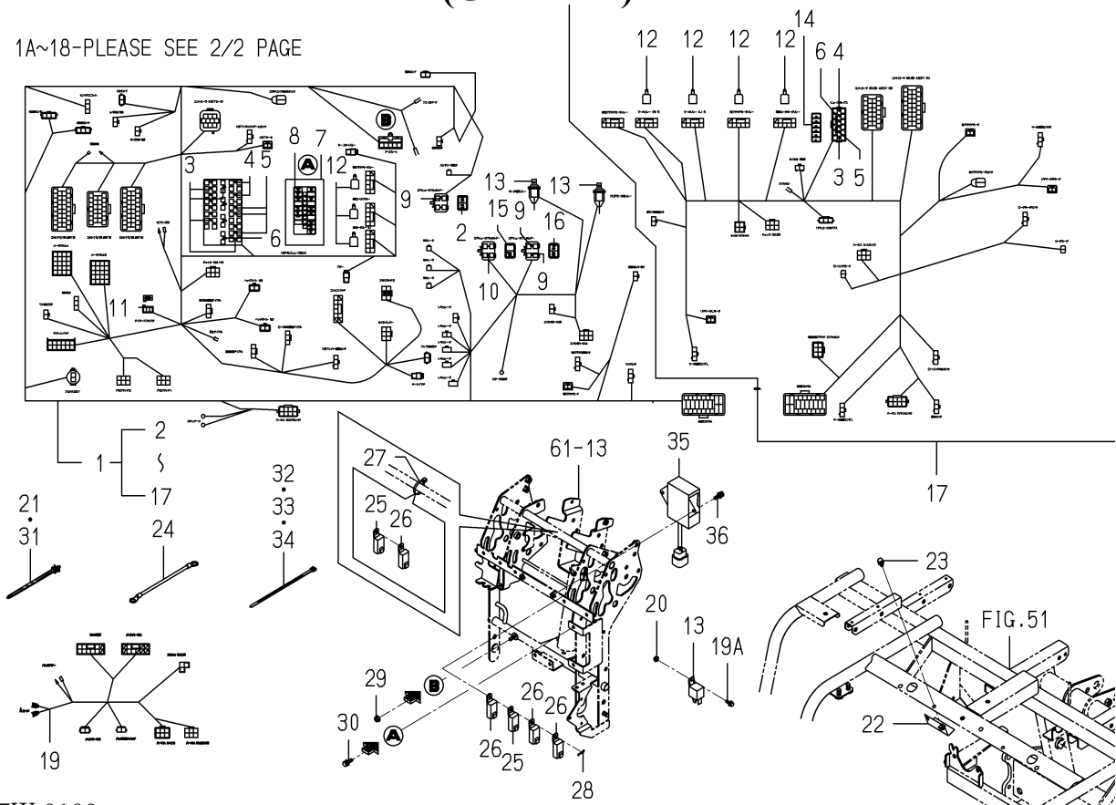
FIG.103 HARNESS(TRAVELING SECTION)SYSTEM(1/2) (GF TYPE)
