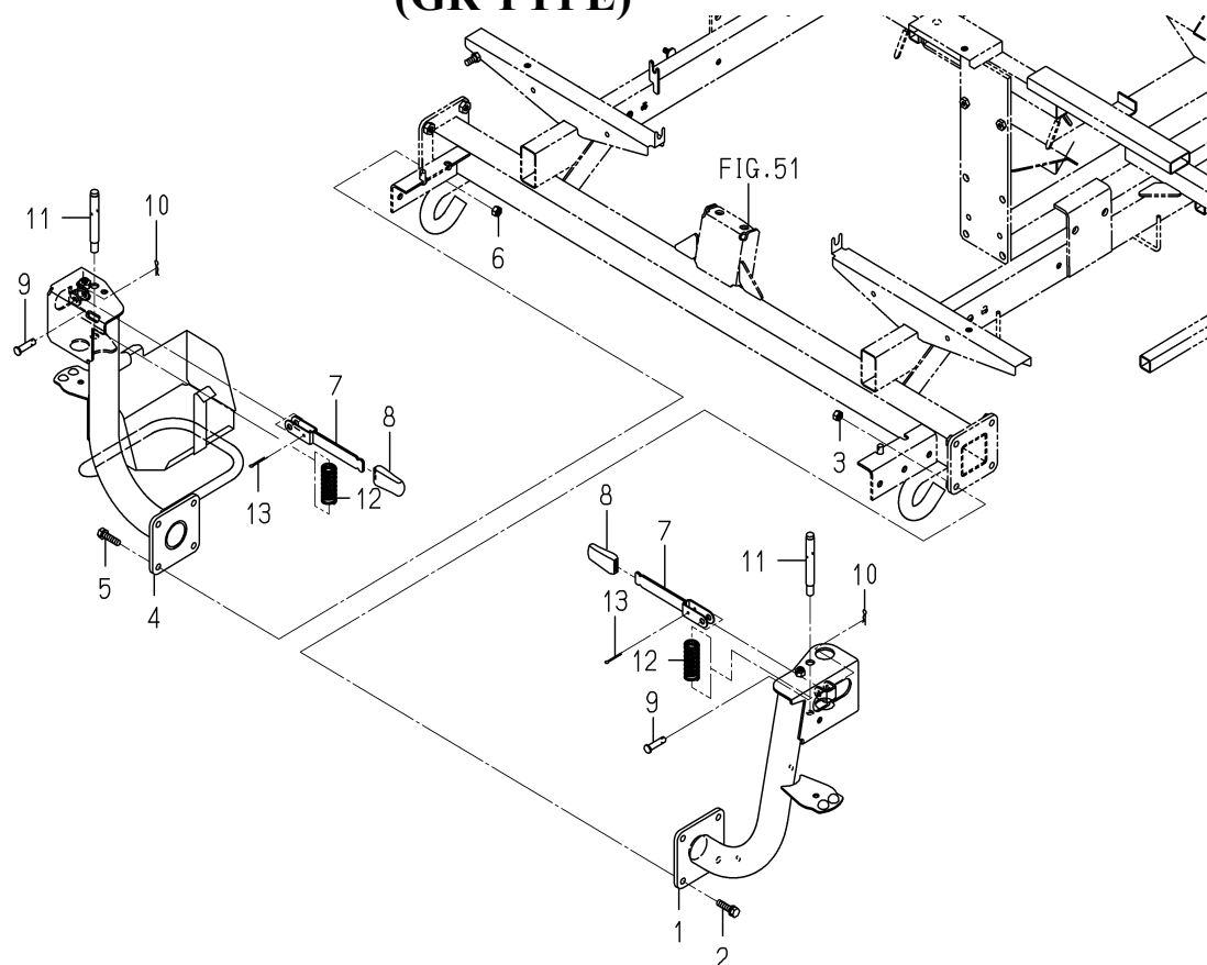
FIG. 90 STAY(FRAME/SEEDLING/SUB)SYSTEM (GR TYPE)
