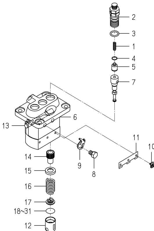
FIG. 29 COMPONENT PARTS FOR 6215-600-156-20 ON Fig.022
