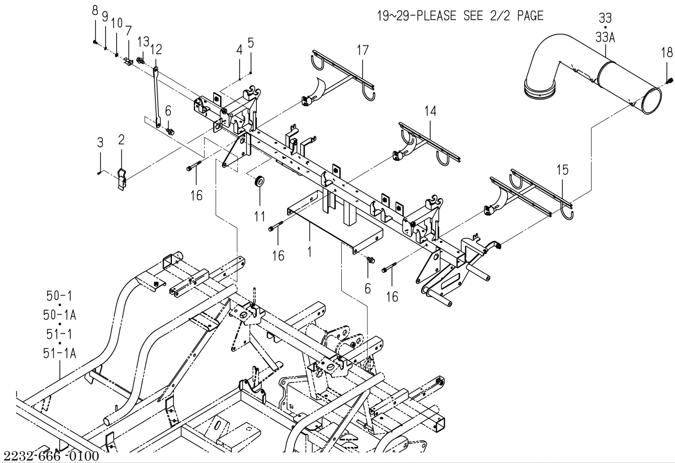
FIG.134 FRAME(FERTILIZER)SYSTEM(F TYPE)(1/2)
