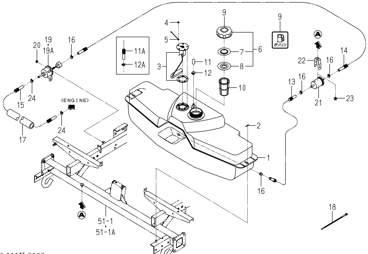
FIG. 12 TANK(FUEL)SYSTEM(G TYPE)
