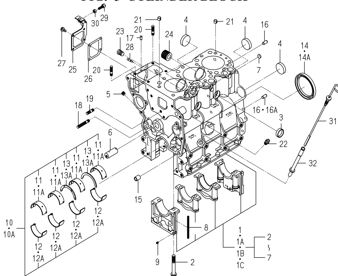
FIG. 5 CYLINDER BLOCK
