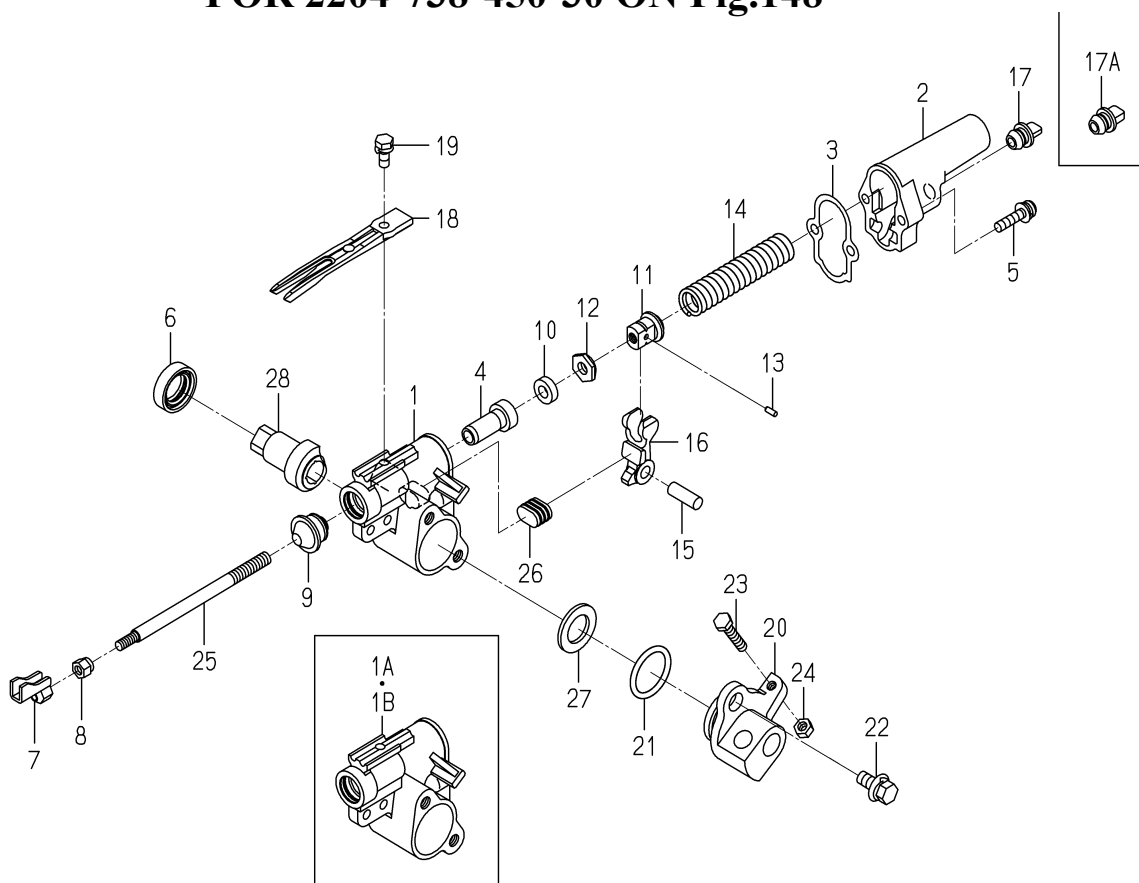
FIG.174 COMPONENT PARTS FOR 2204-738-450-30 ON Fig.148
