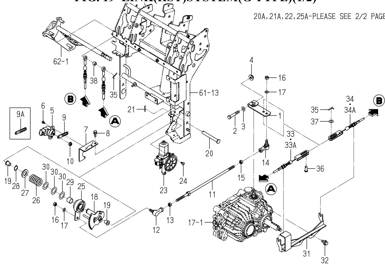
FIG. 19 LINK(HST)SYSTEM(G TYPE)(1/2)
