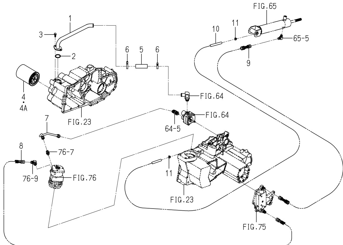
FIG. 66 PIPING SYSTEM
