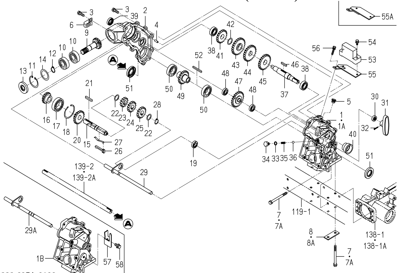
FIG.121 SLIDE SYSTEM(D TYPE)
