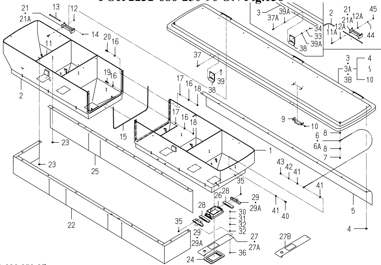
FIG.177 COMPONENT PARTS FOR 2232-686-250-90 ON Fig.136
