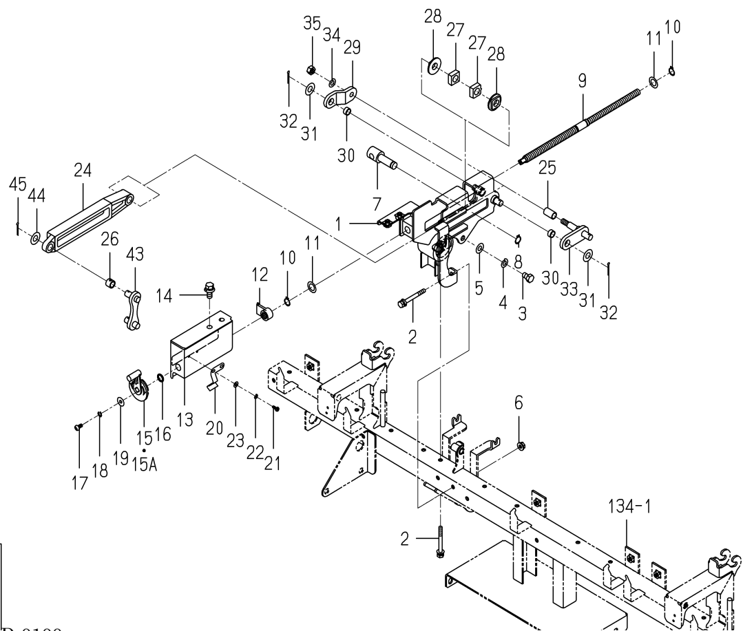
FIG.131 DRIVE(FERTILIZER)SYSTEM(DF TYPE)(1/2)
