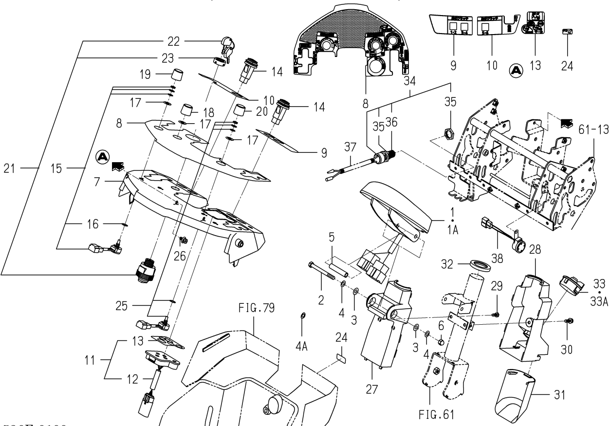
FIG.100 PANEL(INSTRUMENT)SYSTEM(1/2) (G TYPE EXCEPT R)
