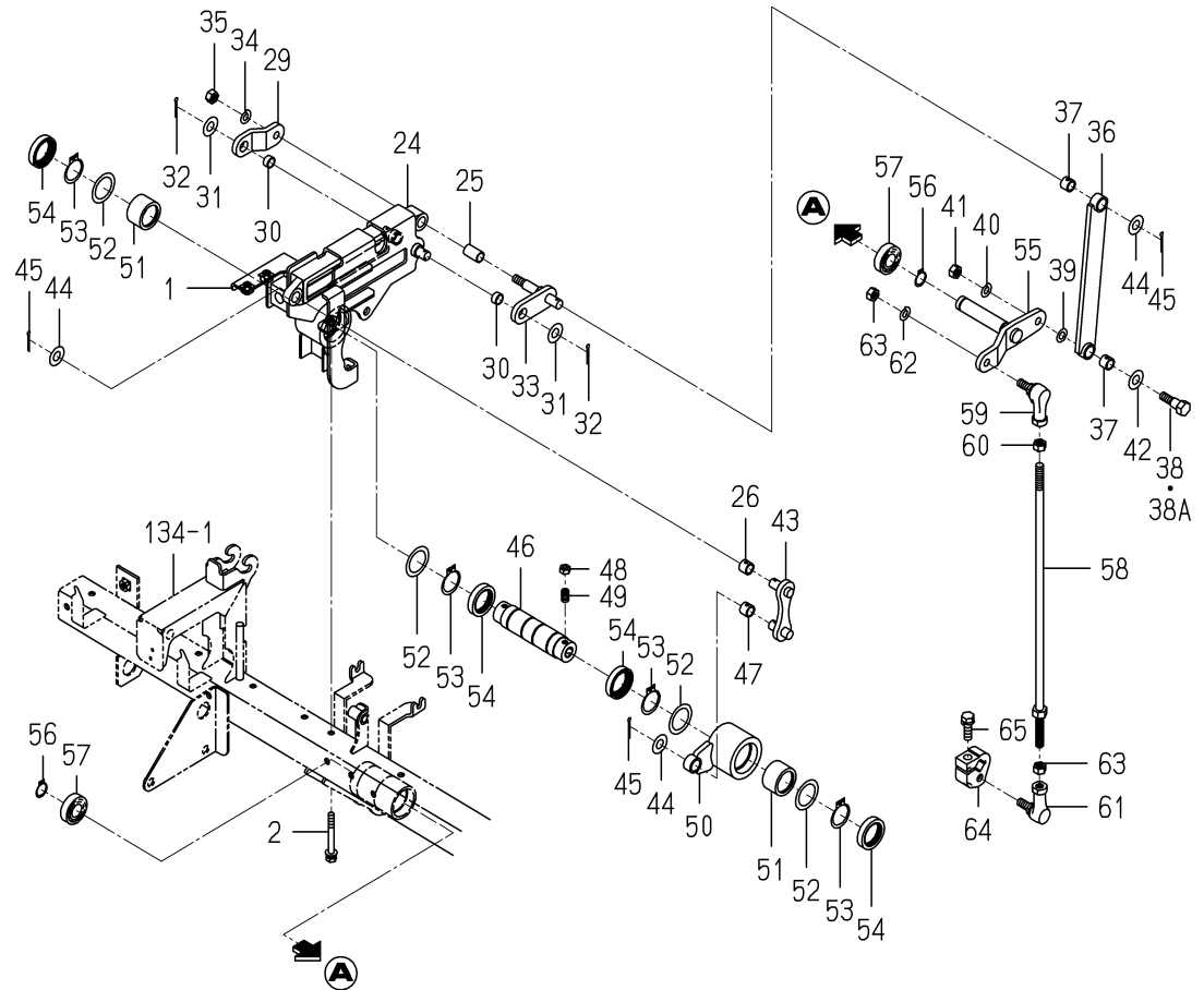
FIG.131 DRIVE(FERTILIZER)SYSTEM(DF TYPE)(2/2)
