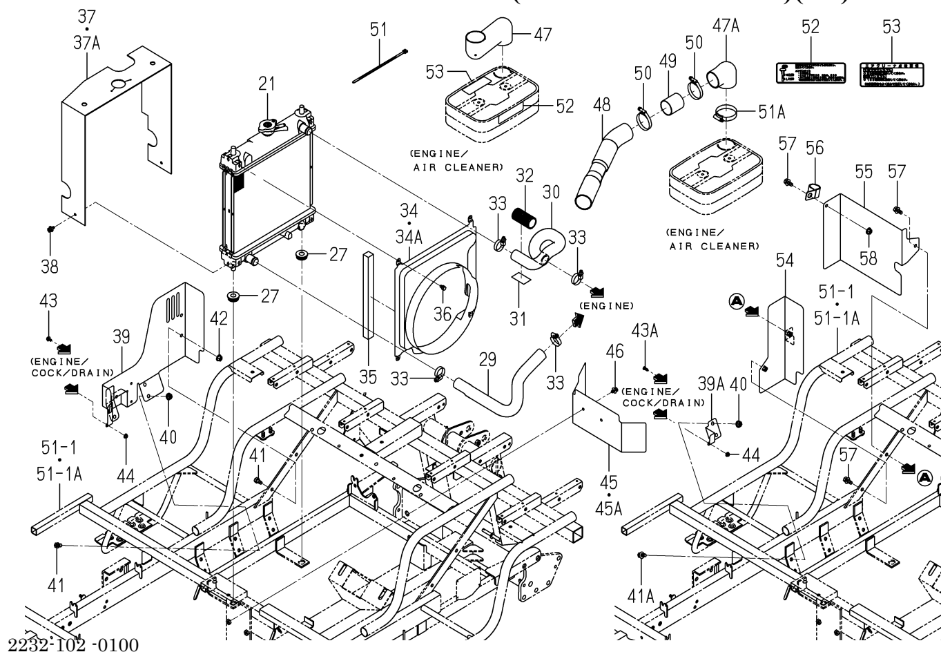
FIG. 3 RADIATOR SYSTEM(G TYPE EXCEPT R)(2/2)
