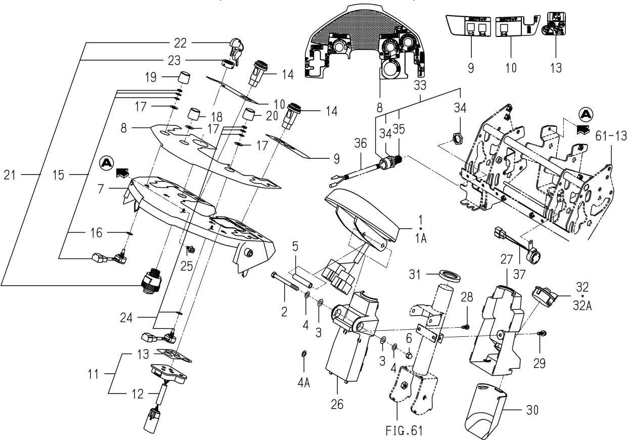
FIG. 99 PANEL(INSTRUMENT)SYSTEM(1/2) (D TYPE EXCEPT R)
