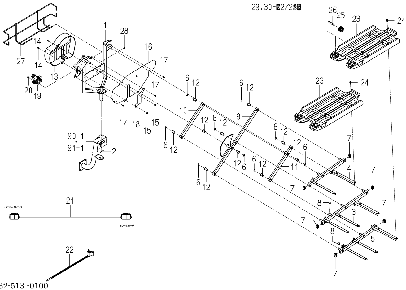
FIG. 87 FRAME(SEEDLING/SUB)SYSTEM(RF TYPE)(1/2)
