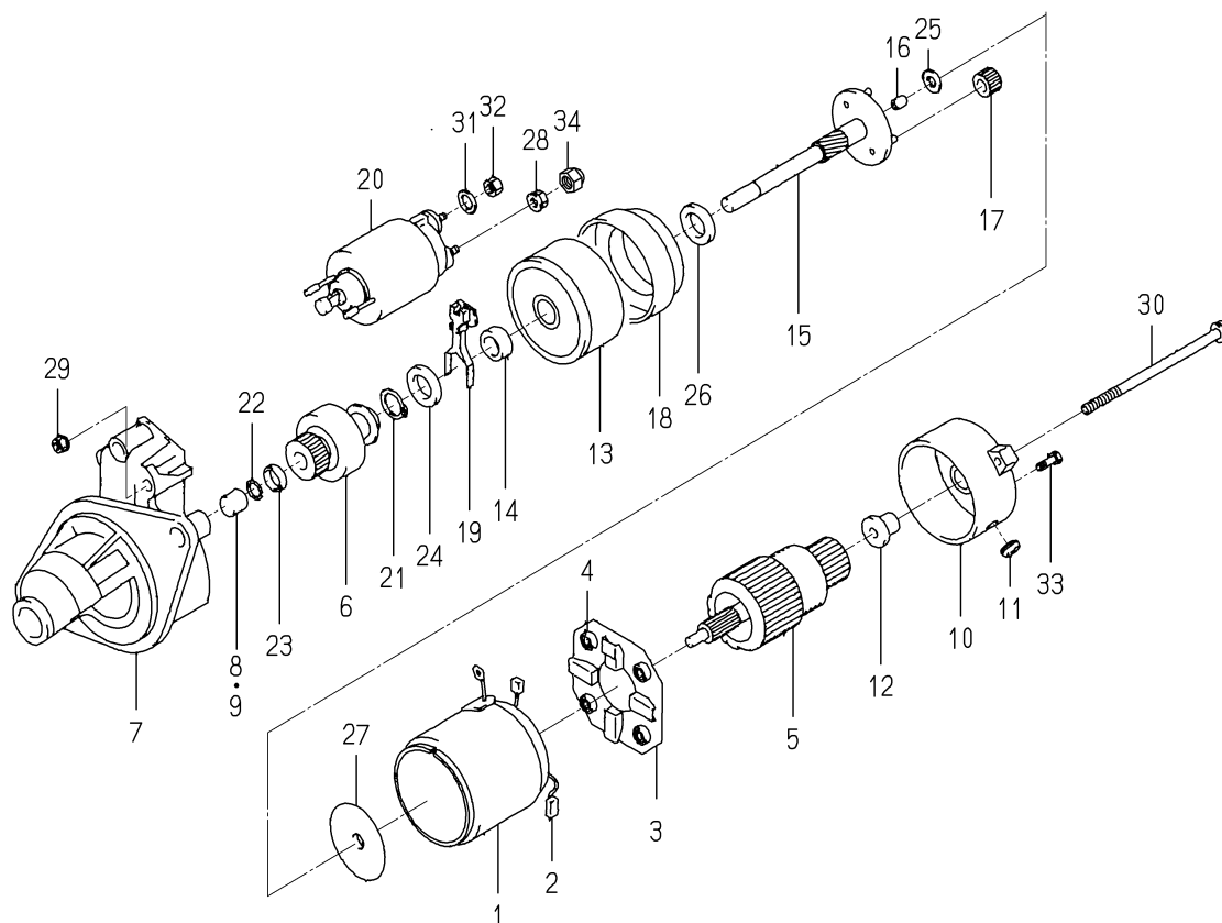
FIG. 30 COMPONENT PARTS FOR 6281-100-014-00 ON Fig.025
