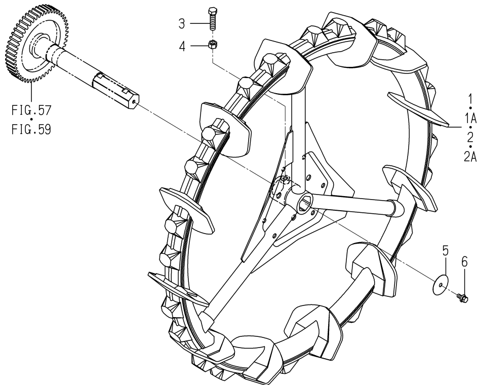
FIG. 41 WHEEL(REAR/900)SYSTEM(G TYPE)
