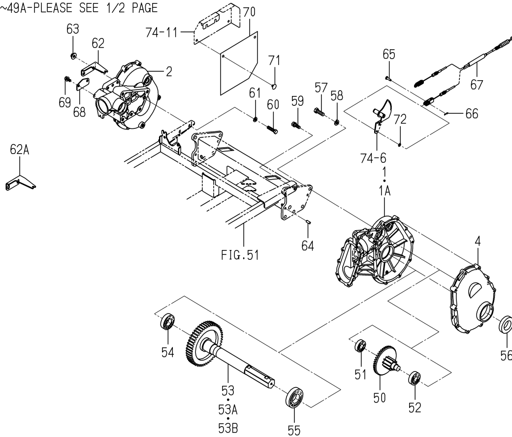
FIG. 57 CASE(REAR)SYSTEM(GF TYPE)(2/2)
