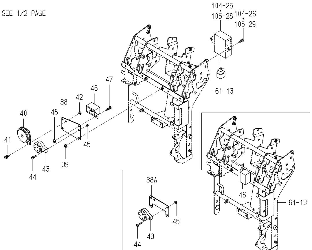
FIG. 99 PANEL(INSTRUMENT)SYSTEM(2/2) (D TYPE EXCEPT R)
