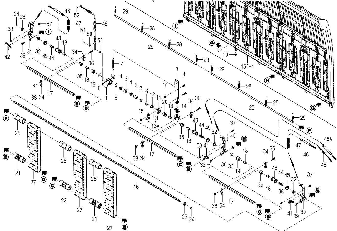
FIG.155 FEED(SEEDLING)SYSTEM
