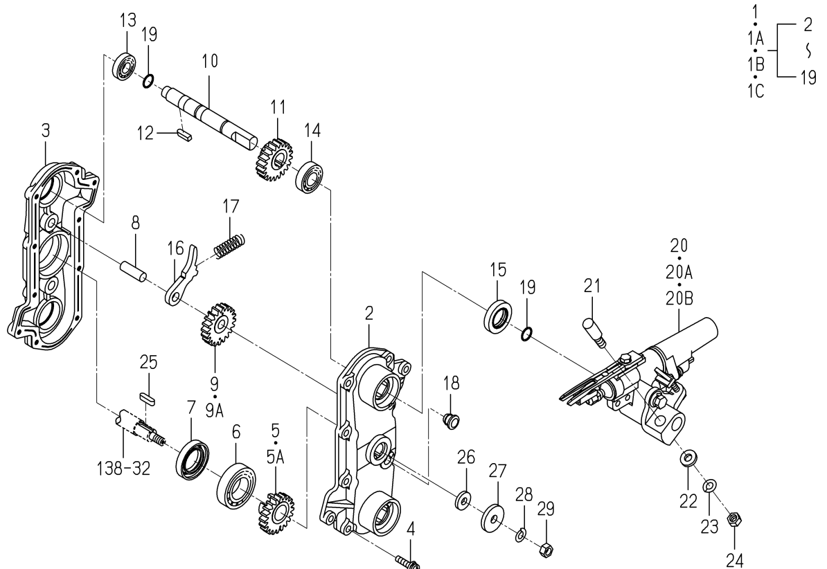
FIG.148 PLANTER(LH)SYSTEM
