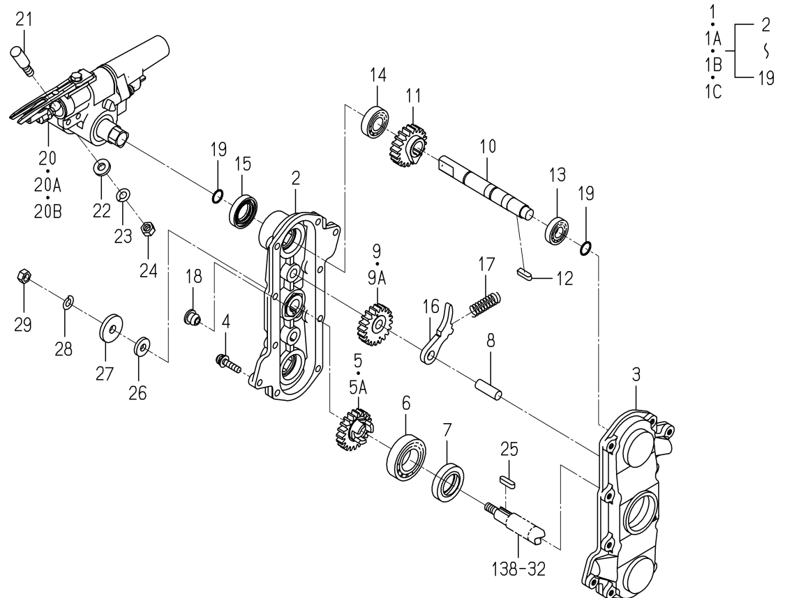
FIG.149 PLANTER(RH)SYSTEM
