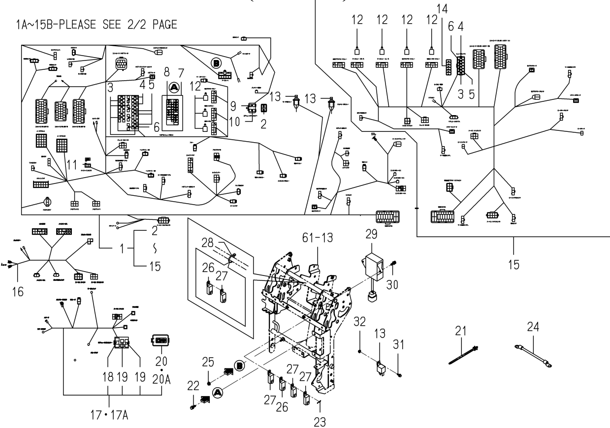
FIG.105 HARNESS(TRAVELING SECTION)SYSTEM(1/2) (DF TYPE)
