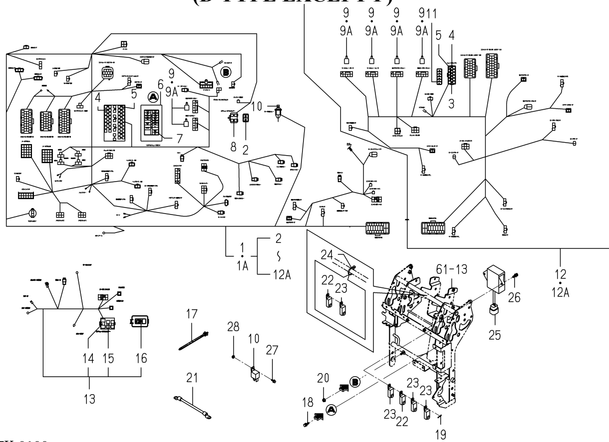
FIG.104 HARNESS(TRAVELING SECTION)SYSTEM (D TYPE EXCEPT F)
