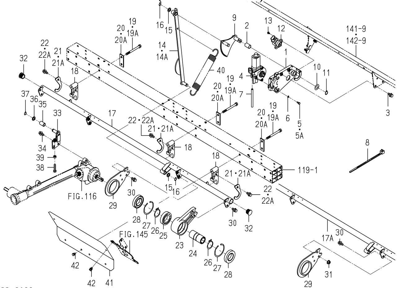
FIG.115 LEVER(DEPTH/ROTOR)SYSTEM
