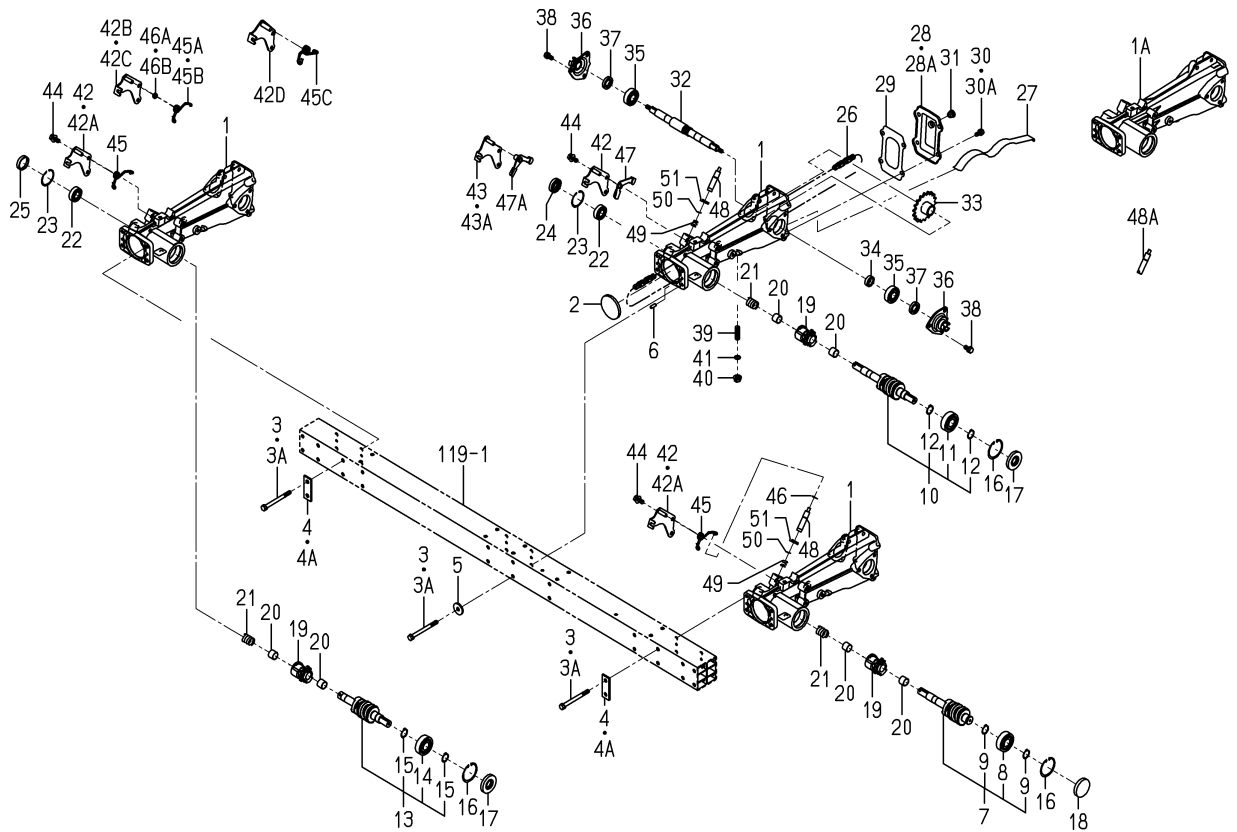
FIG.138 FRAME(SIDE)SYSTEM
