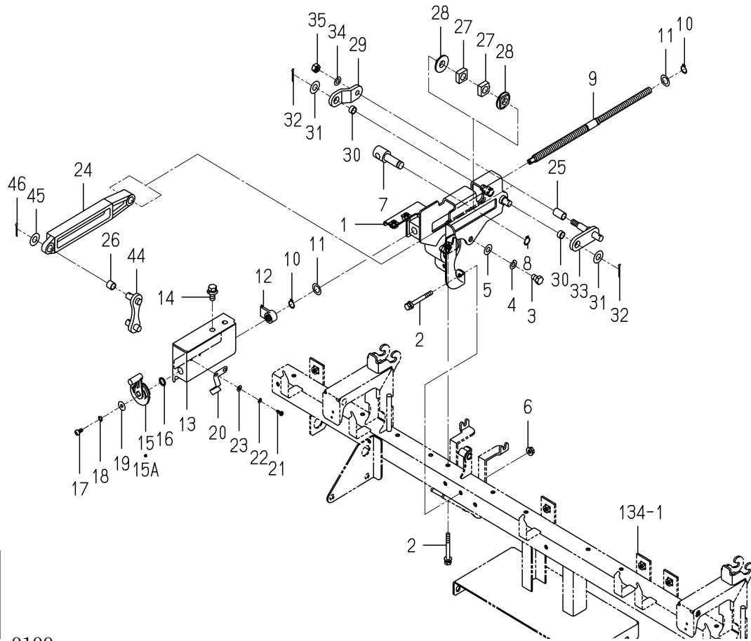
FIG.130 DRIVE(FERTILIZER)SYSTEM(GF TYPE)(1/2)
