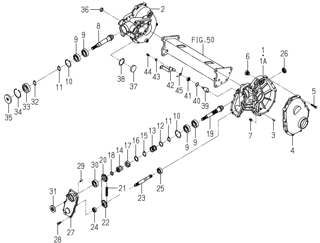
FIG. 60 CASE(REAR)SYSTEM(DF TYPE)(1/2)
