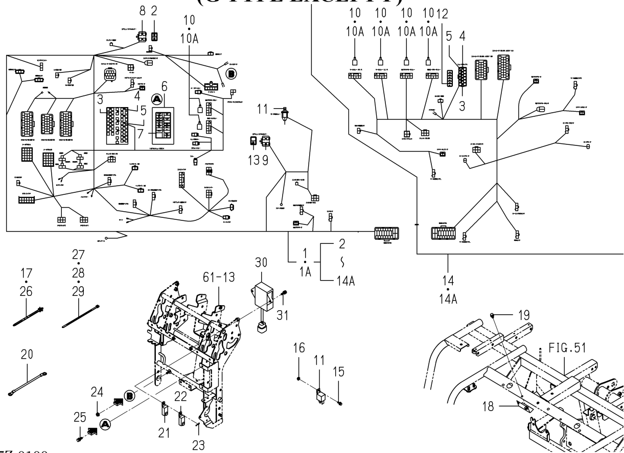
FIG.106 HARNESS(TRAVELING SECTION)SYSTEM (G TYPE EXCEPT F)
