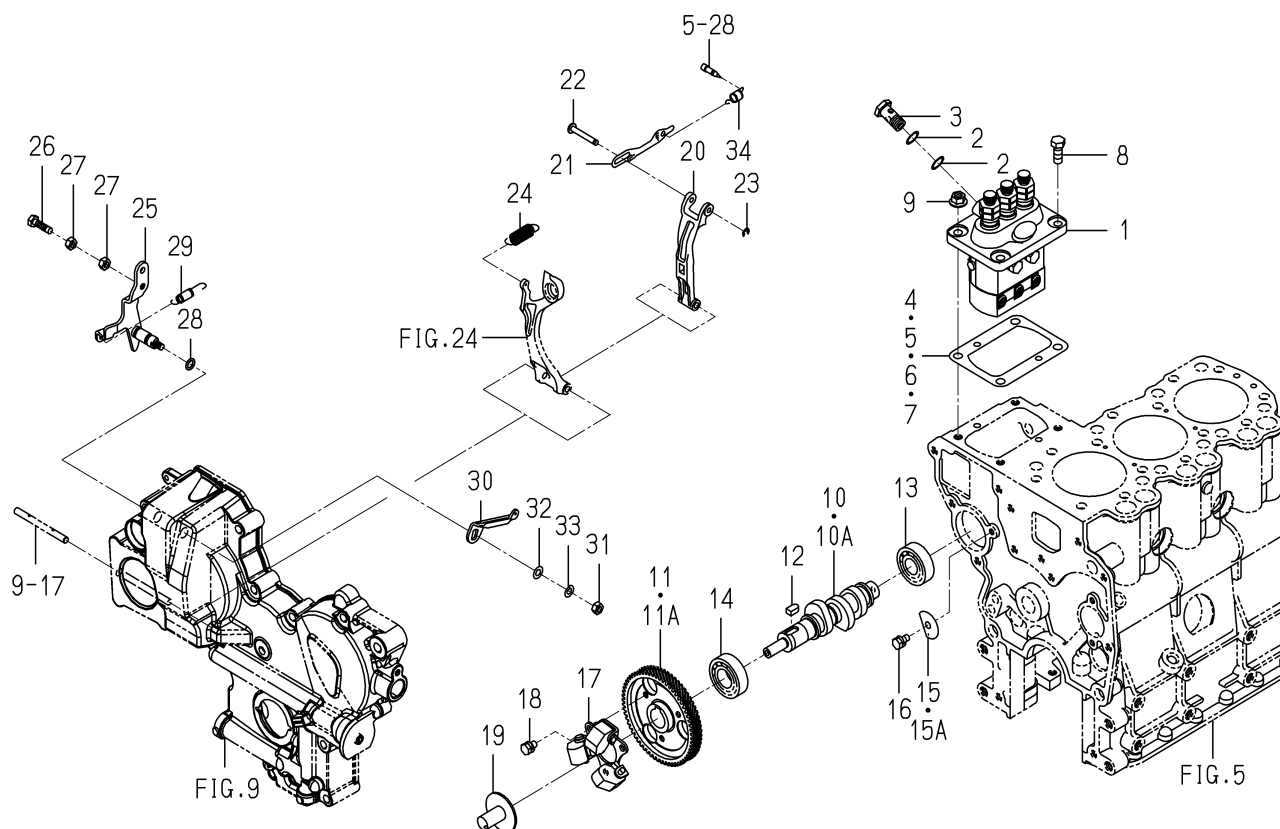
FIG. 22 INJECTION PUMP
