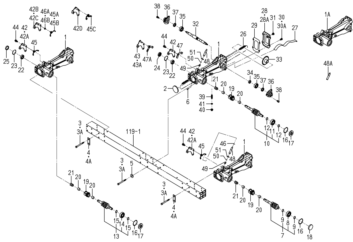
FIG.138 FRAME(SIDE)SYSTEM
