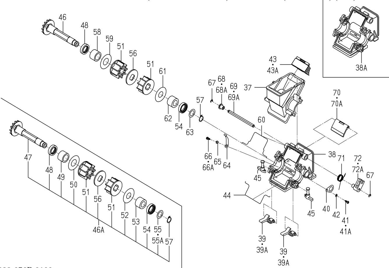
FIG.135 SEND OUT(FERTILIZER)SYSTEM(F TYPE)(2/3)
