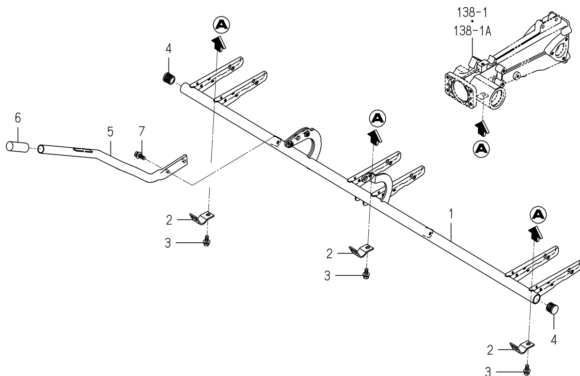
FIG.125 LEVER(DEPTH/PLANTING)SYSTEM
