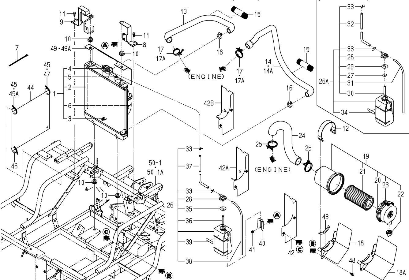
FIG. 4 RADIATOR&CLEANER(AIR)SYSTEM(D TYPE)
