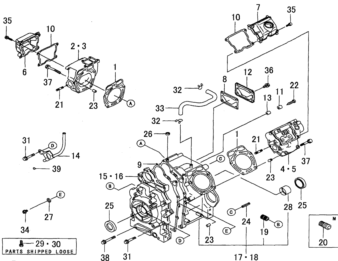
FIG. 1 CYLINDER/CRANKCASE
