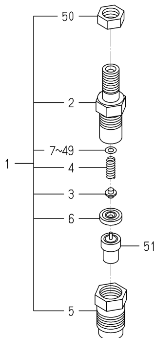
FIG. 28 COMPONENT PARTS FOR 6215-300-036-10 ON Fig.021
