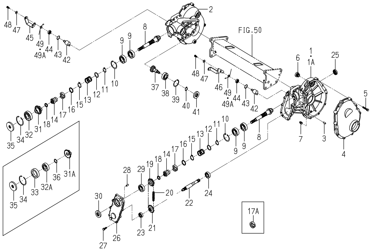
FIG. 58 CASE(REAR)SYSTEM(DF TYPE)(1/2)
