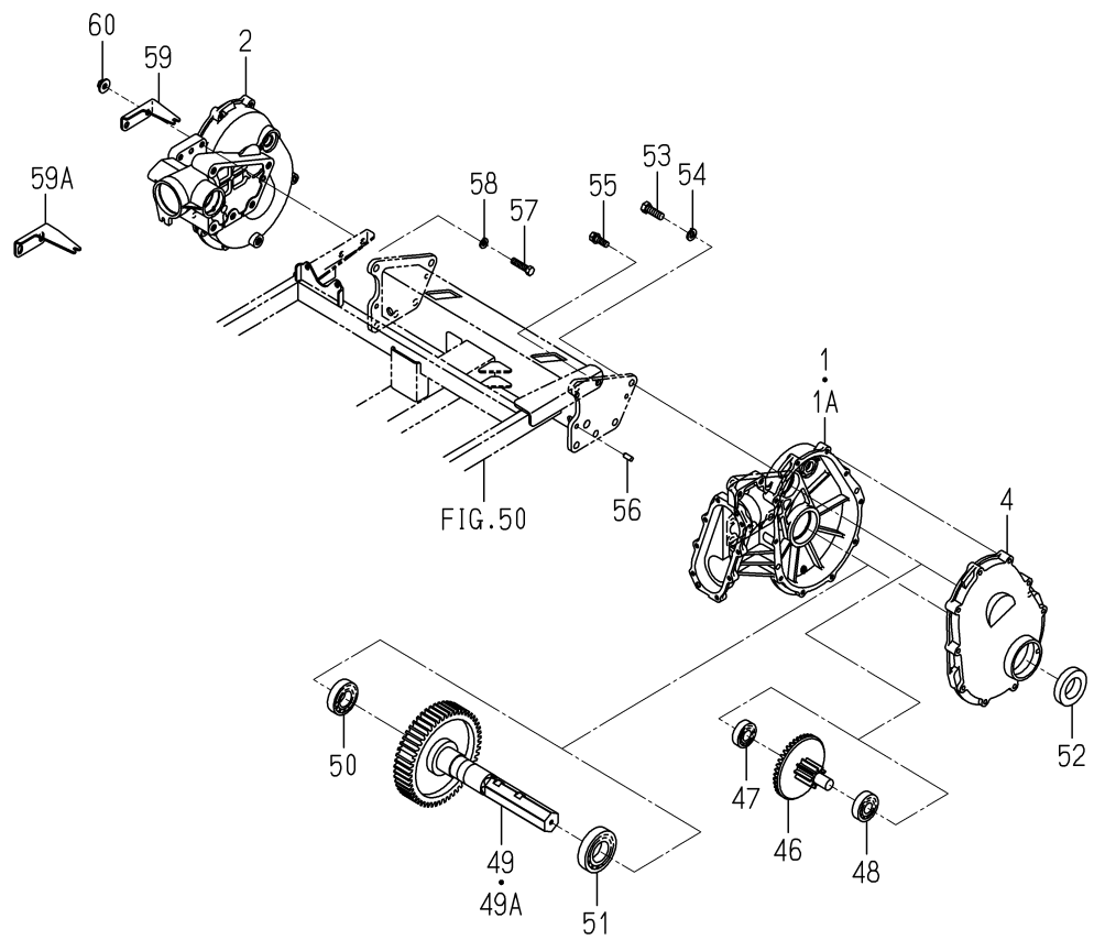
FIG. 60 CASE(REAR)SYSTEM(DF TYPE)(2/2)
