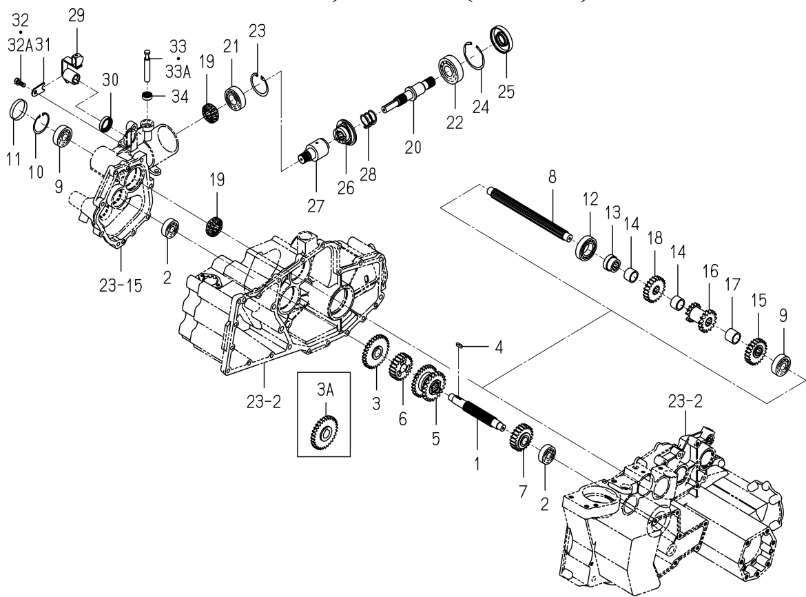
FIG. 35 SHAFT(PLANTING INTERVAL,PLANTING/ OUTPUT)SYSTEM(G TYPE)
