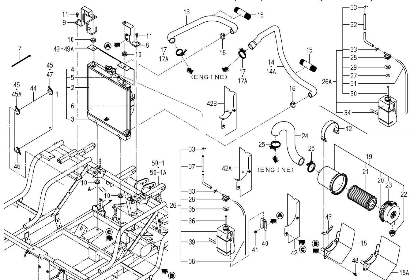
FIG. 4 RADIATOR&CLEANER(AIR)SYSTEM(D TYPE)
