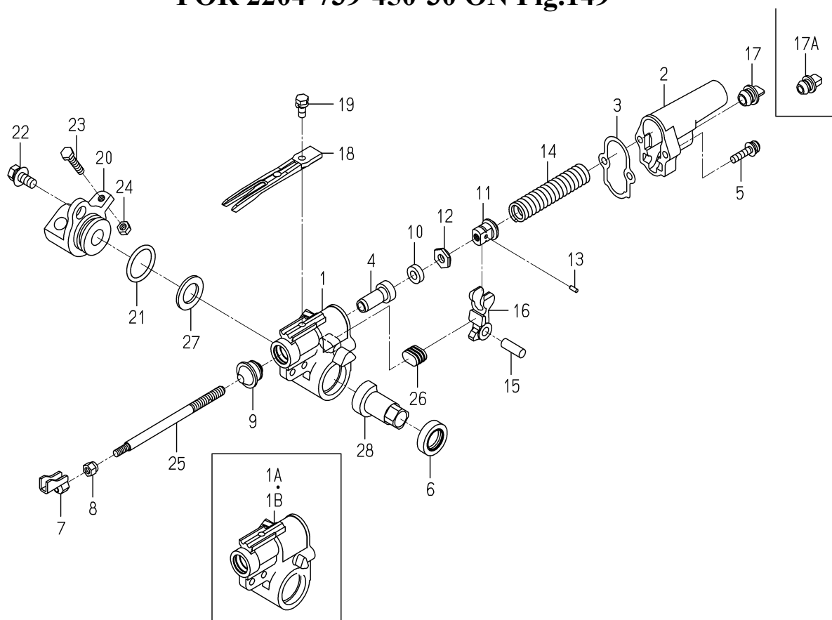
FIG.175 COMPONENT PARTS FOR 2204-739-450-30 ON Fig.149
