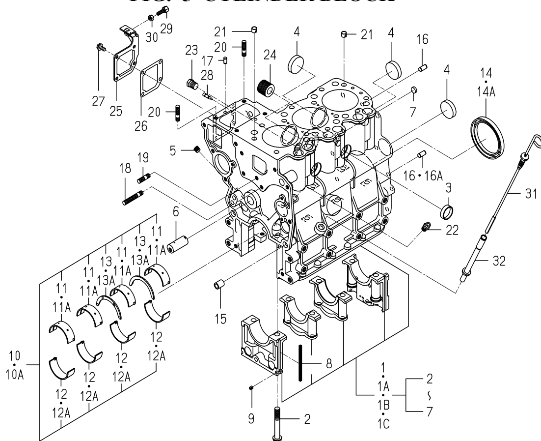
FIG. 5 CYLINDER BLOCK
