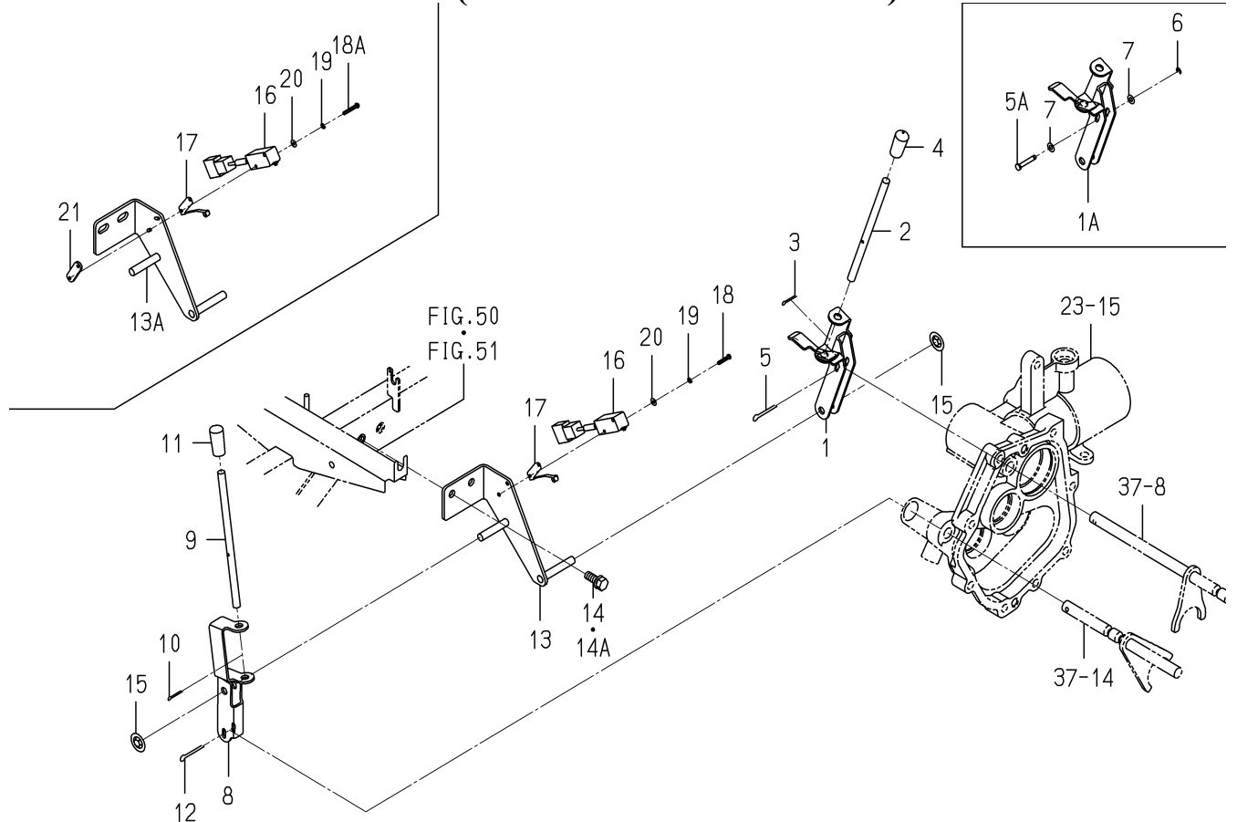
FIG. 38 LEVER(PLANTING INTERVAL)SYSTEM
