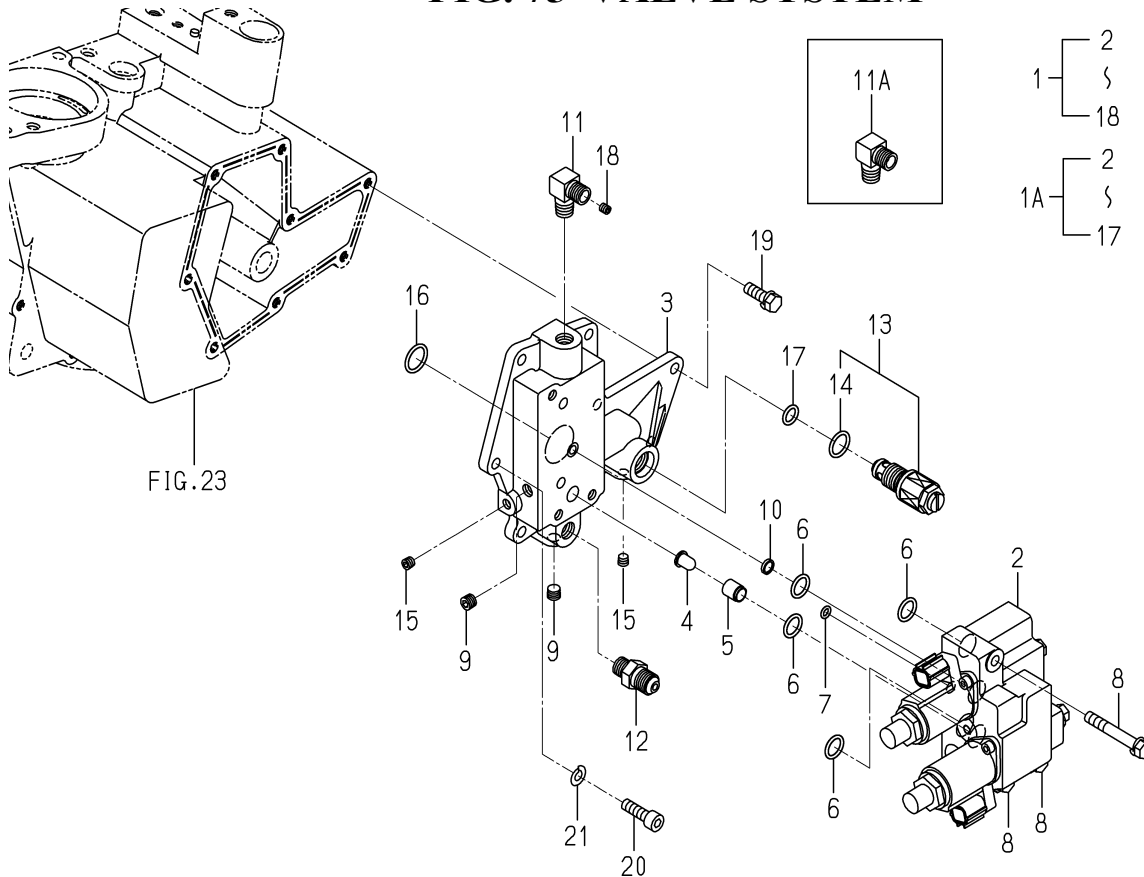
FIG. 75 VALVE SYSTEM
