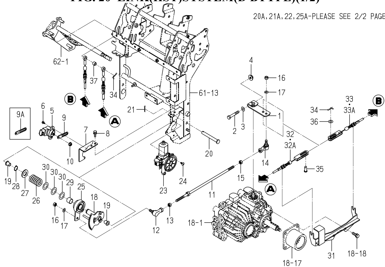
FIG. 20 LINK(HST)SYSTEM(D BTYPE)(1/2)
