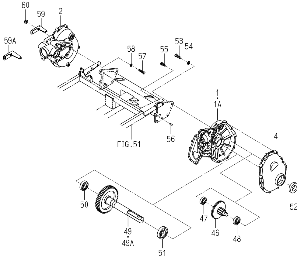
FIG. 59 CASE(REAR)SYSTEM(GF TYPE)(2/2)
