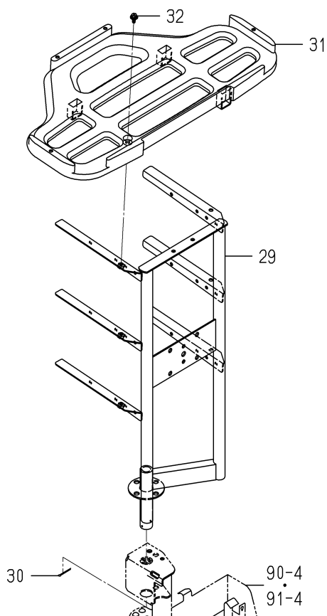
FIG. 88 FRAME(SEEDLING/SUB)SYSTEM(2/2) (R TYPE EXCEPT F)
