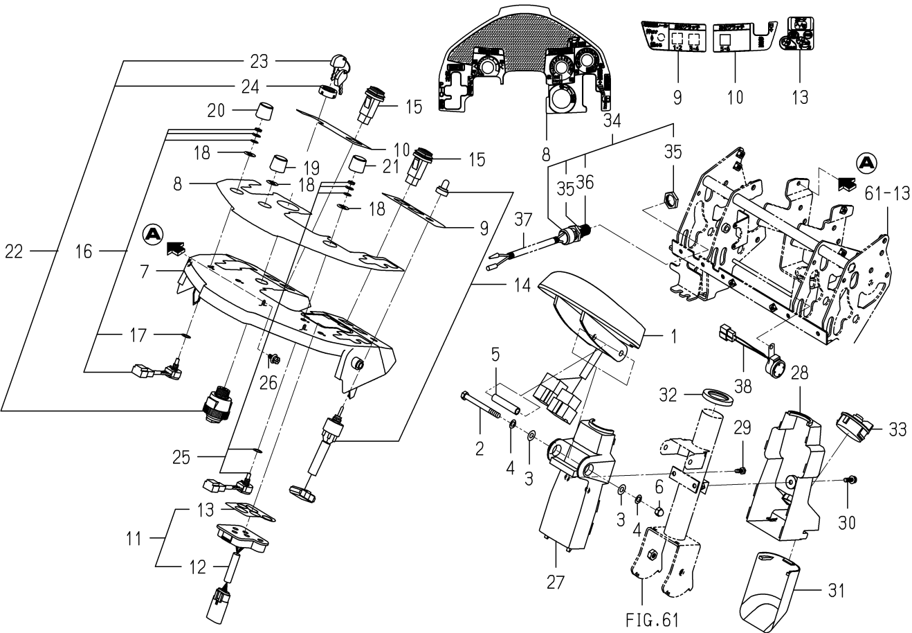
FIG.101 PANEL(INSTRUMENT)SYSTEM(GR TYPE)(1/2)
