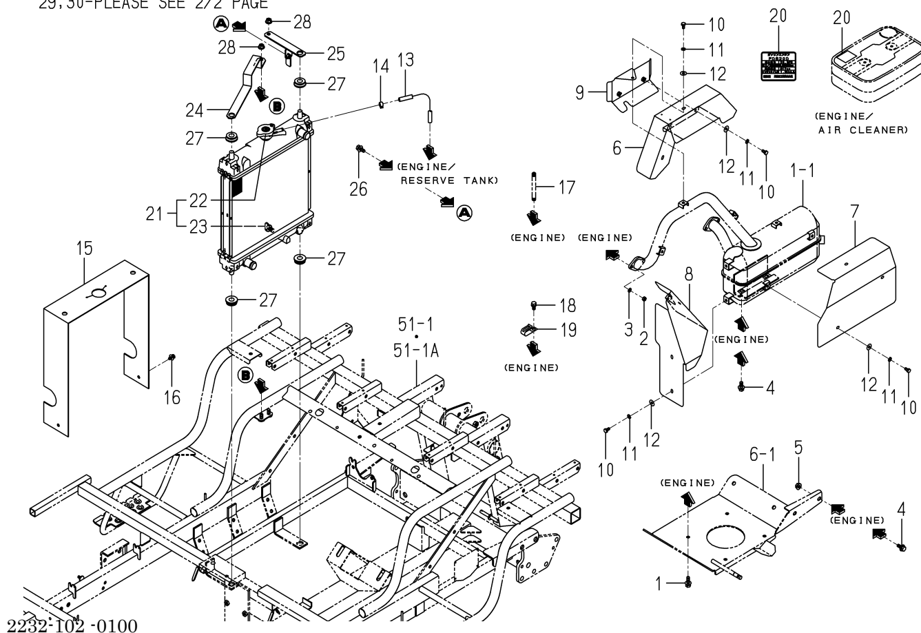
FIG. 3 RADIATOR SYSTEM(G TYPE EXCEPT R)(1/2)
