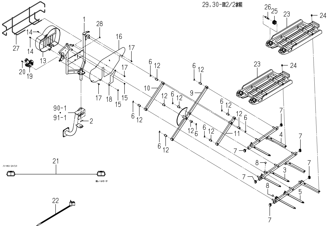
FIG. 88 FRAME(SEEDLING/SUB)SYSTEM(1/2) (R TYPE EXCEPT F)
