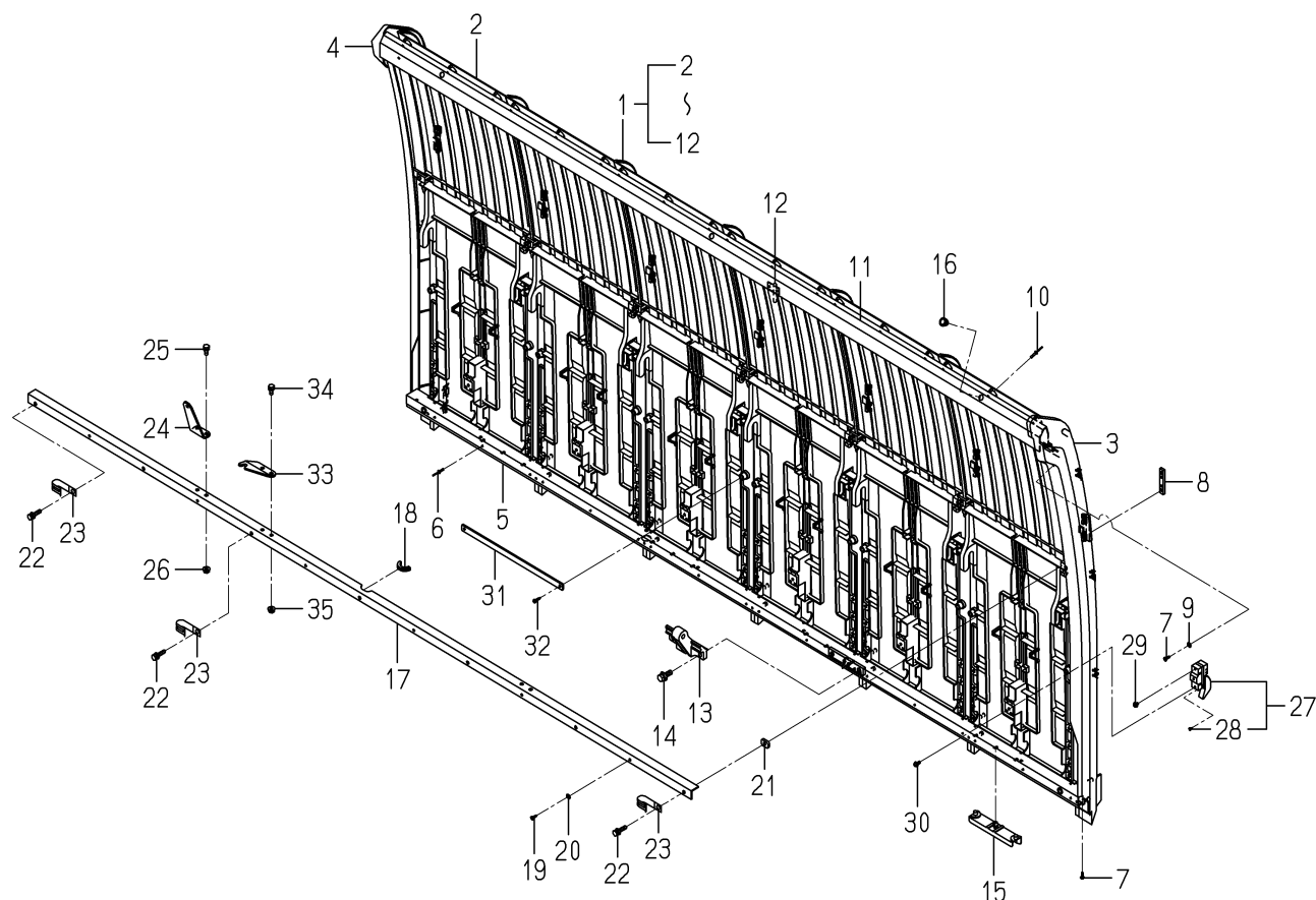
FIG.150 TANK(SEEDLING)SYSTEM
