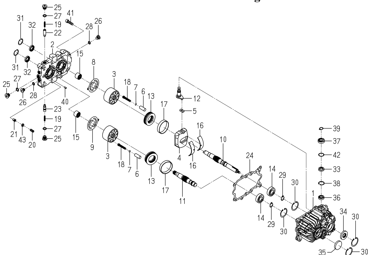
FIG.173 COMPONENT PARTS FOR K510-022-000-00 ON Fig.18
