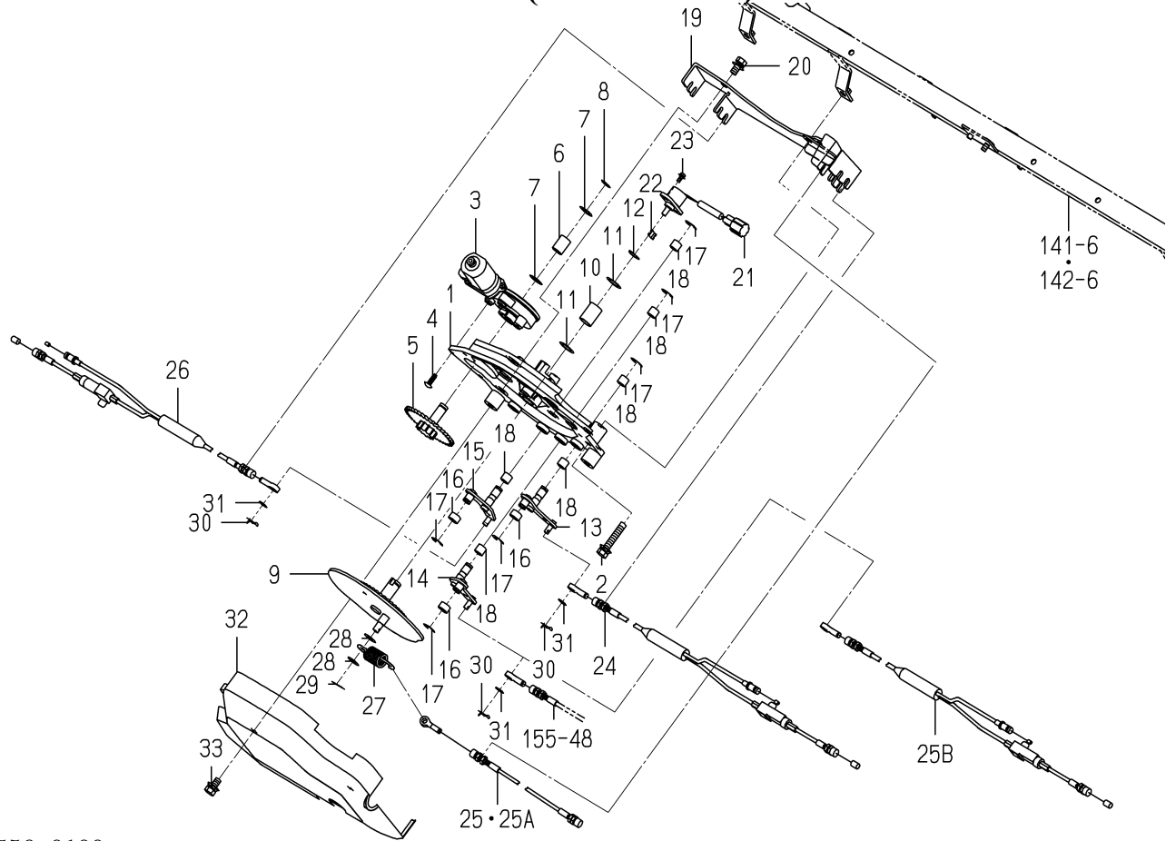
FIG.112 CLUTCH(PLANTING)SYSTEM
