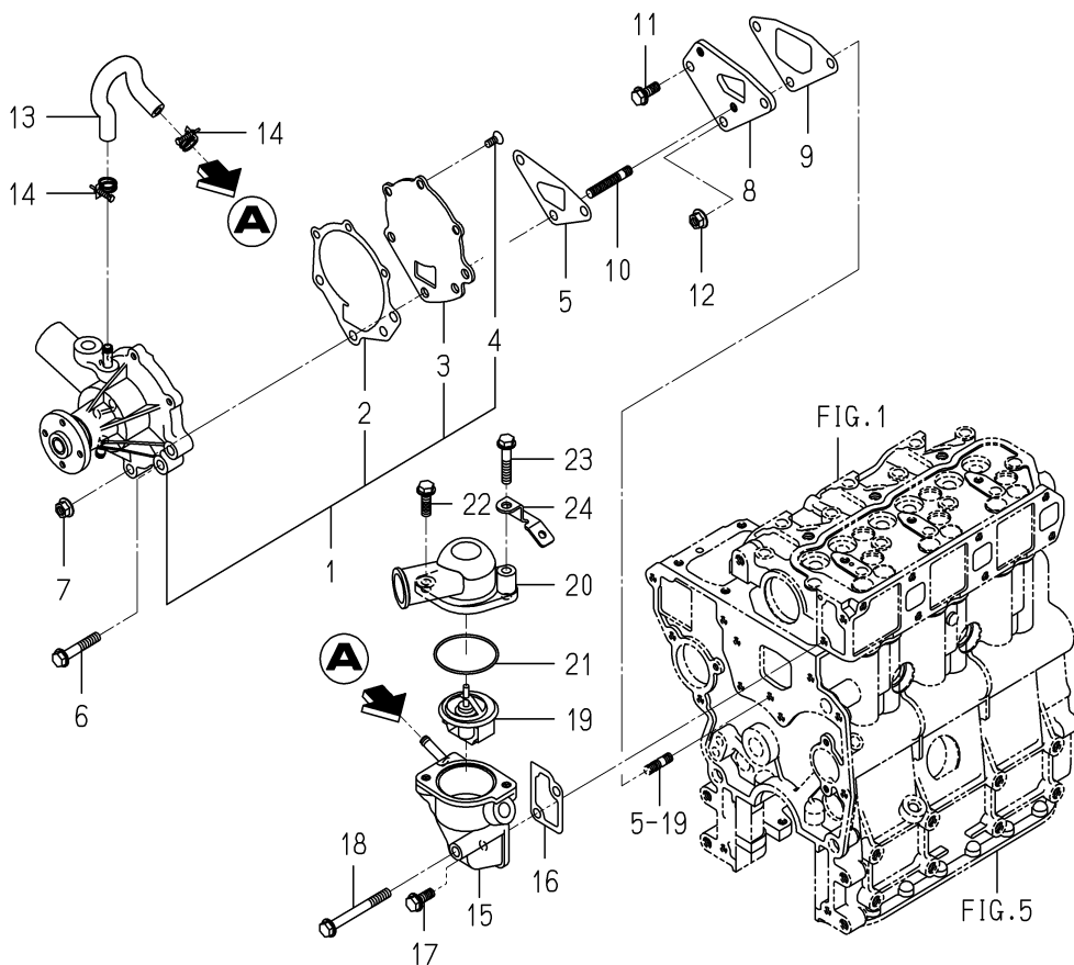
FIG. 18 WATER PUMP
