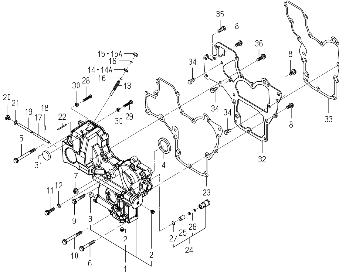
FIG. 9 TIMING GEAR CASE
