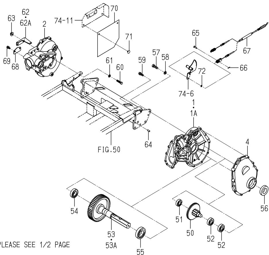
FIG. 58 CASE(REAR)SYSTEM(DF TYPE)(2/2)
