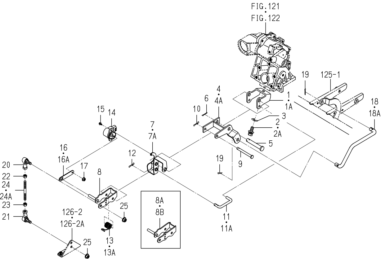
FIG.120 LINK(FLOAT)SYSTEM
