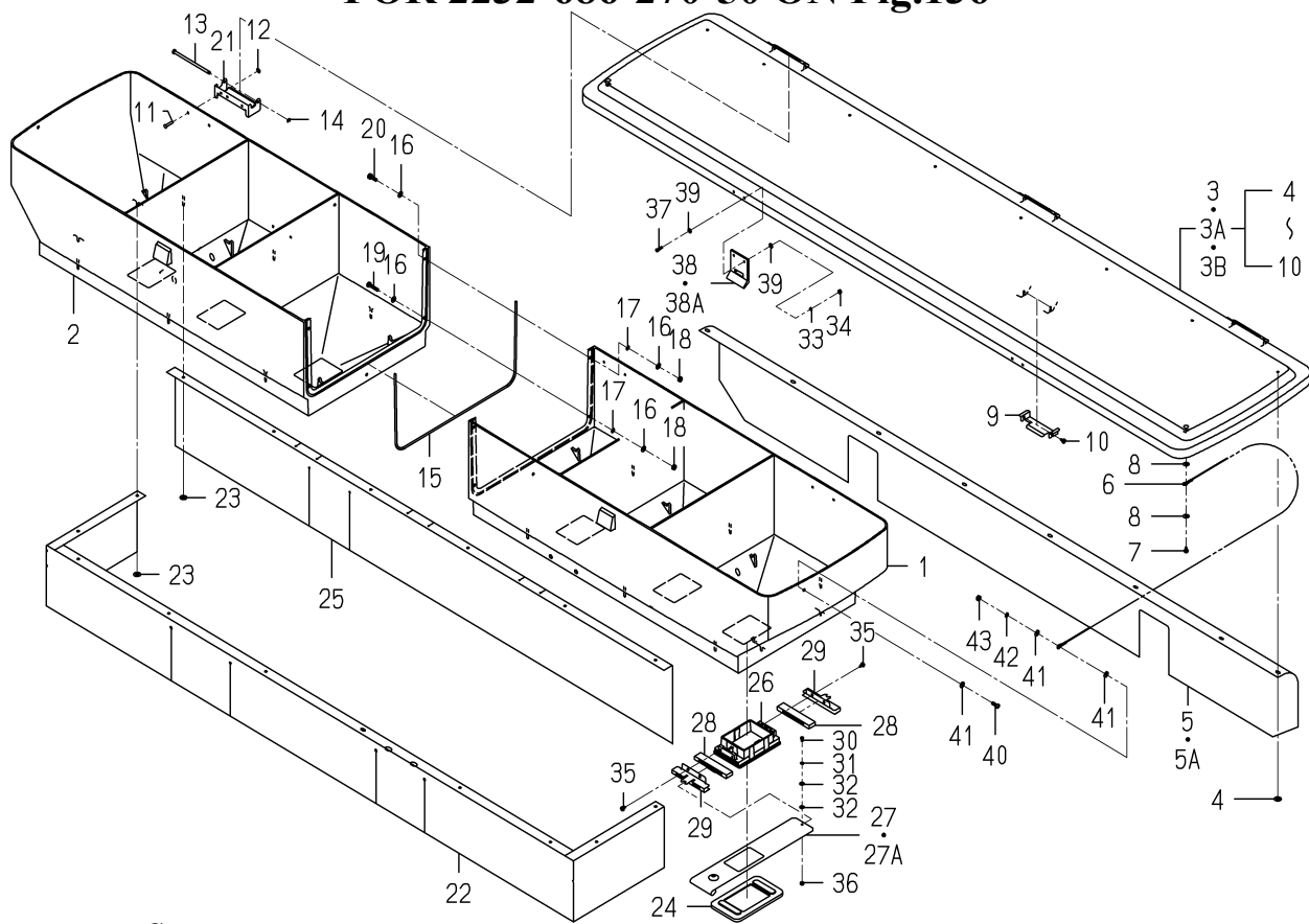
FIG.178 COMPONENT PARTS FOR 2232-686-270-50 ON Fig.136
