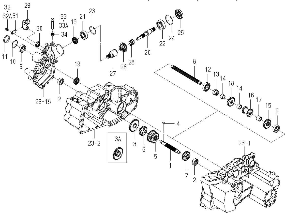
FIG. 36 SHAFT(PLANTING INTERVAL, PLANTING/OUTPUT)SYSTEM(D TYPE)
