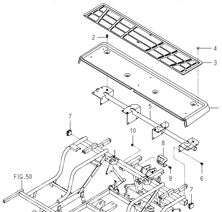
FIG. 84 STEP(REAR)SYSTEM(D TYPE EXCEPT F) (EXCEPT R TYPE-NO.631-)
