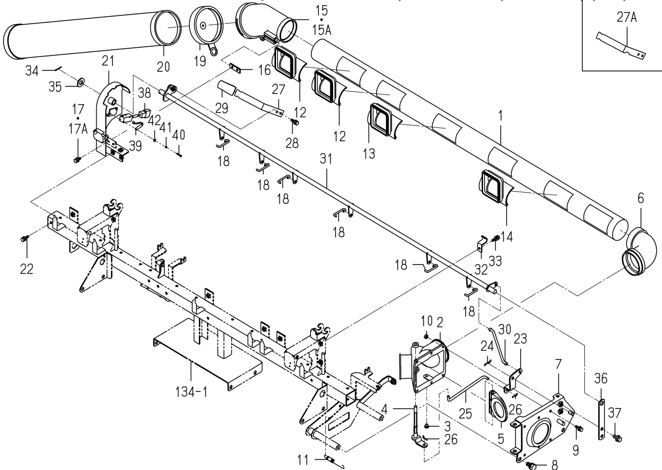
FIG.133 AIR CHAMBER(FERTILIZER)SYSTEM(F TYPE)(1/2)
