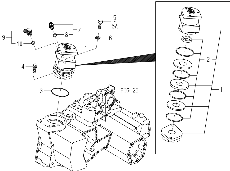
FIG. 76 CONTROLLER(STEERING)SYSTEM (EXCEPT R TYPE)(NO.1-630)
