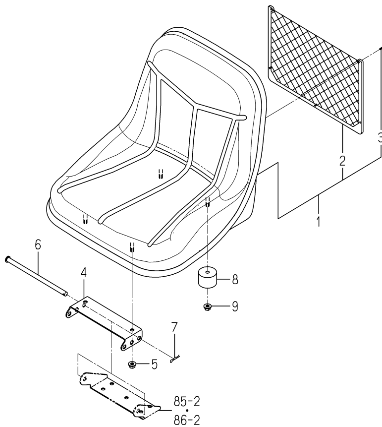
FIG. 95 SEAT SYSTEM
