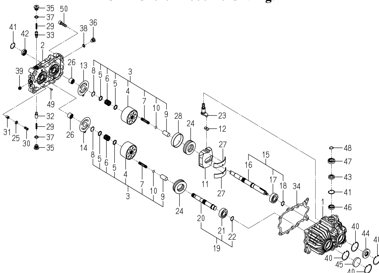
FIG.172 COMPONENT PARTS FOR K510-021-000-20 ON Fig.17
