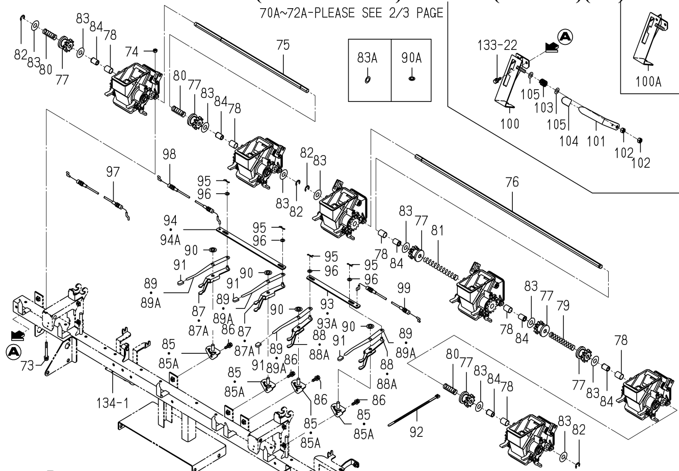
FIG.135 SEND OUT(FERTILIZER)SYSTEM(F TYPE)(3/3)
