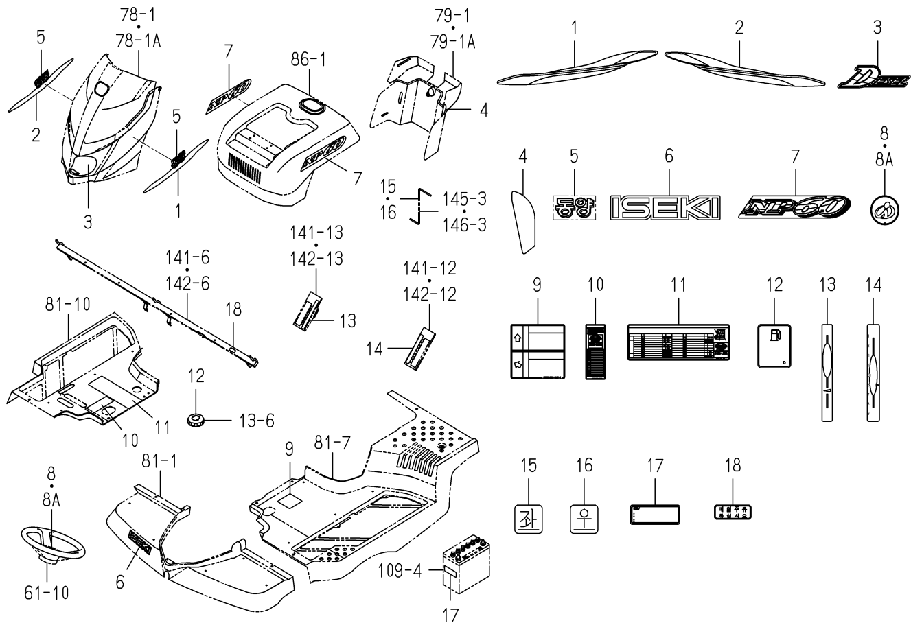
FIG.163 ORNAMENT&LABEL(D TYPE EXCEPT R)
