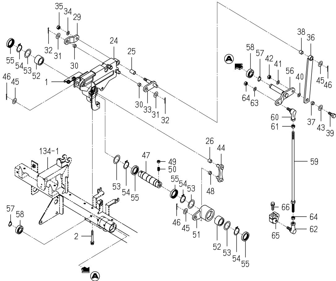
FIG.130 DRIVE(FERTILIZER)SYSTEM(GF TYPE)(2/2)
