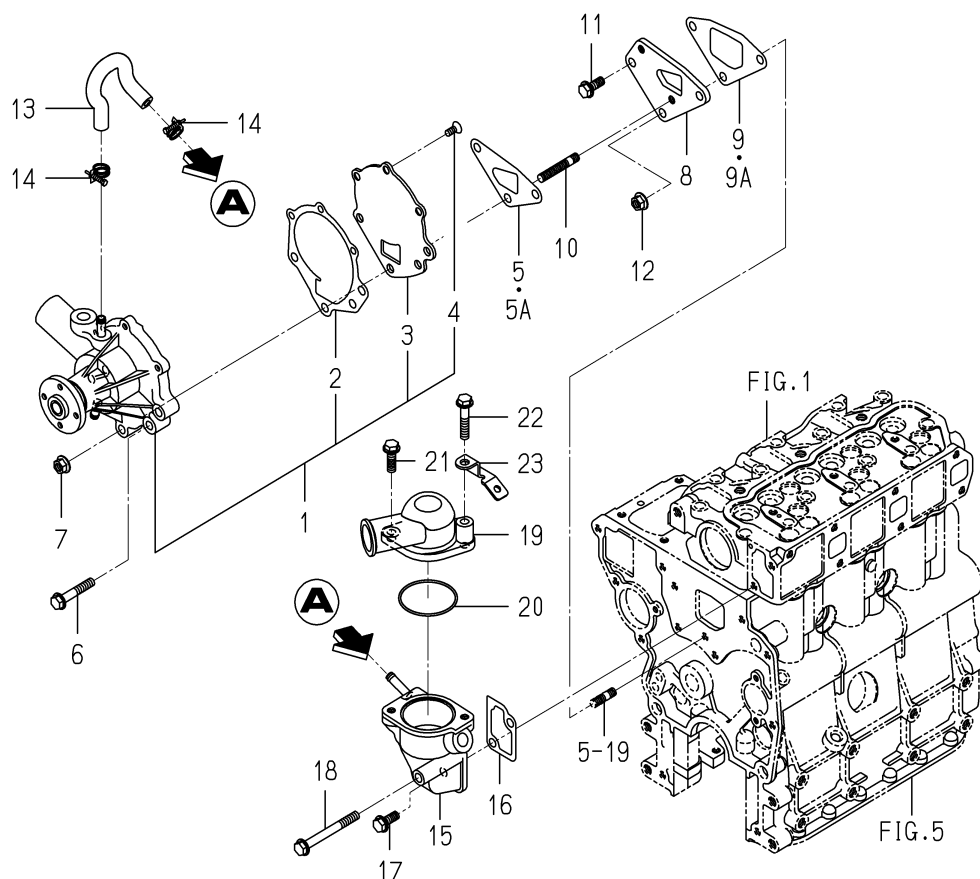
FIG. 19 WATER PUMP
