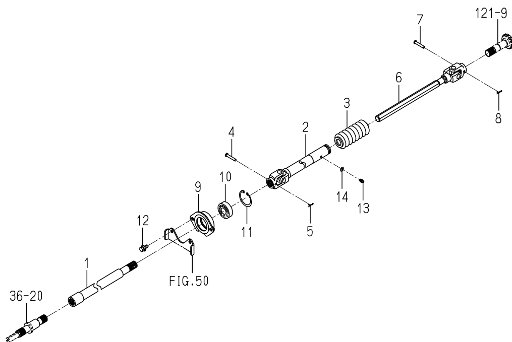
FIG. 54 SHAFT(PLANTING)SYSTEM(D TYPE)
