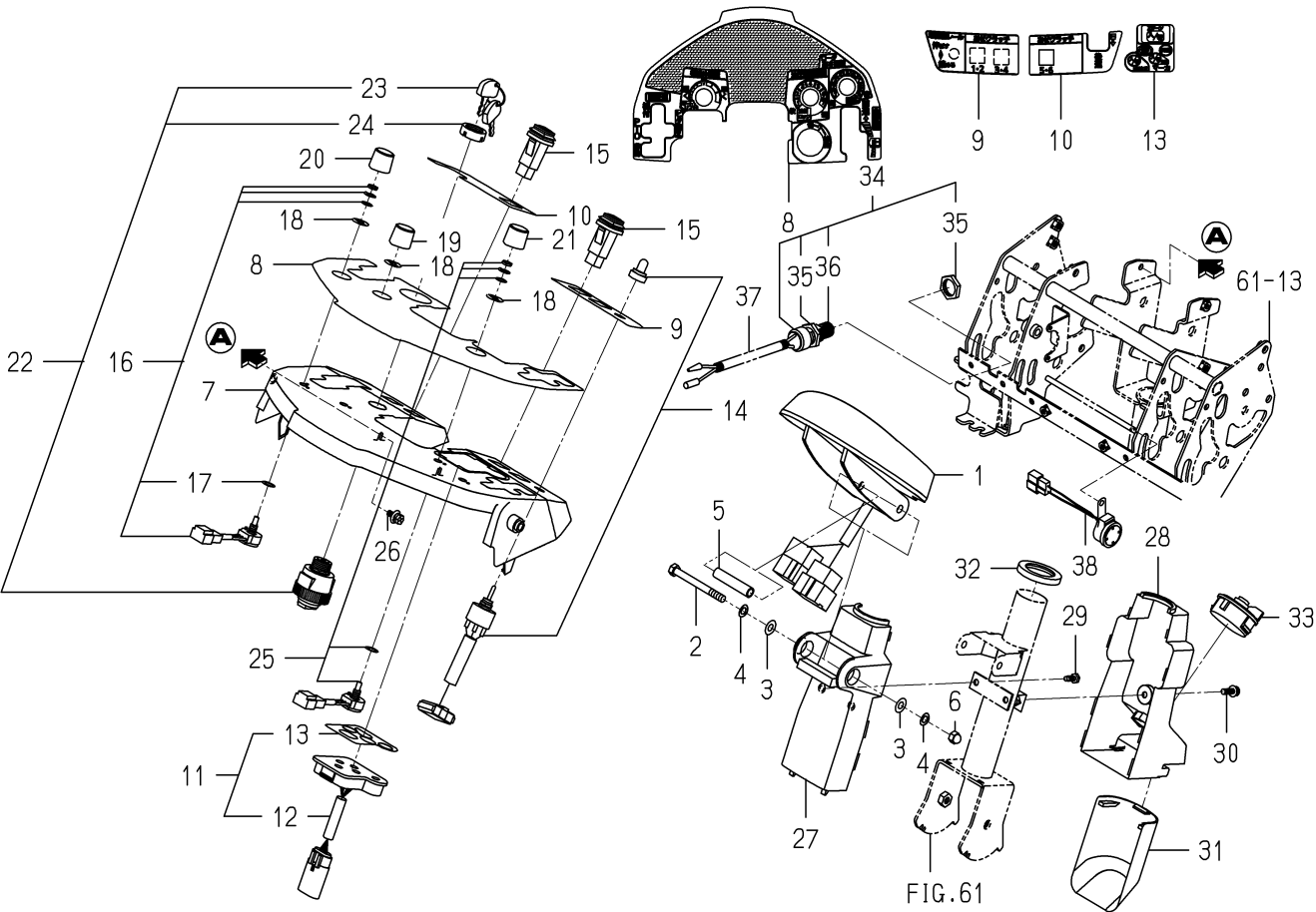
FIG.102 PANEL(INSTRUMENT)SYSTEM(DR TYPE)(1/2)
