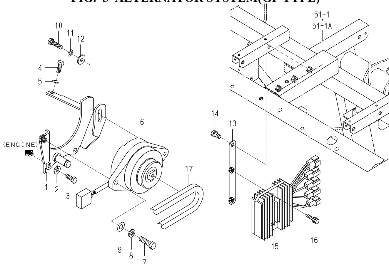
FIG. 5 ALTERNATOR SYSTEM(GF TYPE)
