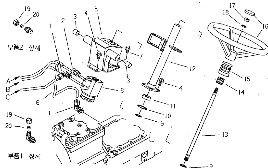
FIG 6-3 STEERING GROUP(630)
