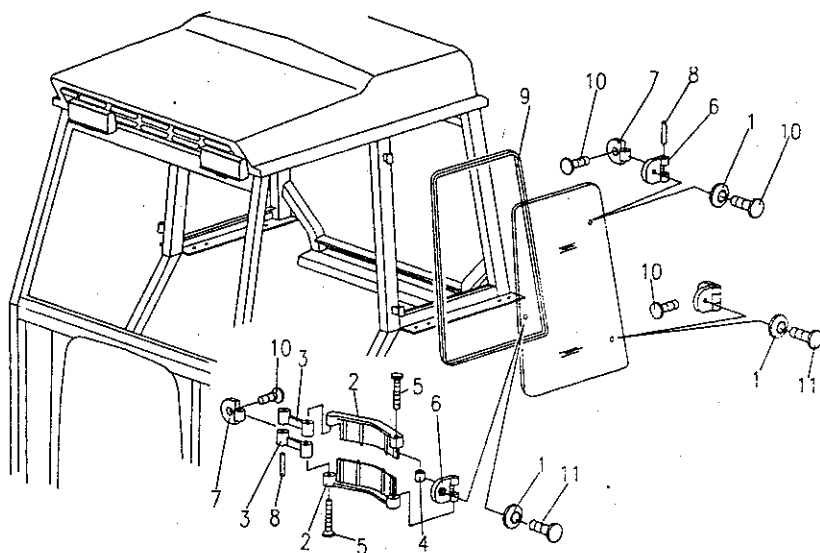
FIG 11-5 옆창문 SIDE WINDOW(862)
