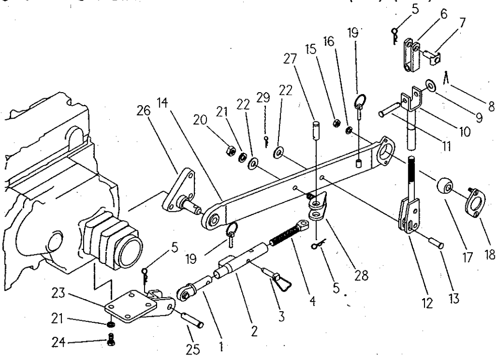
FIG 9-4 3-POINT LINKAGE-LOWER LINK(LH) (896)
