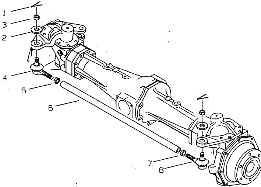
TIE ROD GROUP (610)
