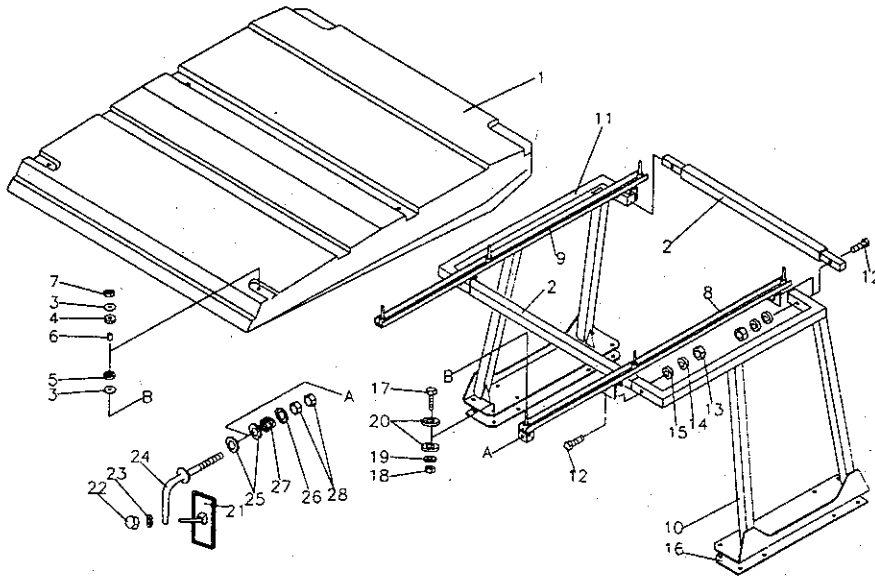
FIG 9-1 SAFETY FRAME & BACK MIRROR (880, 909)
