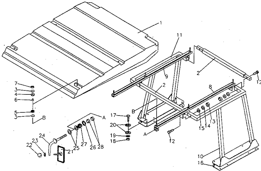
FIG 9-1 SAFETY FRAME & BACK MIRROR (880, 909)
