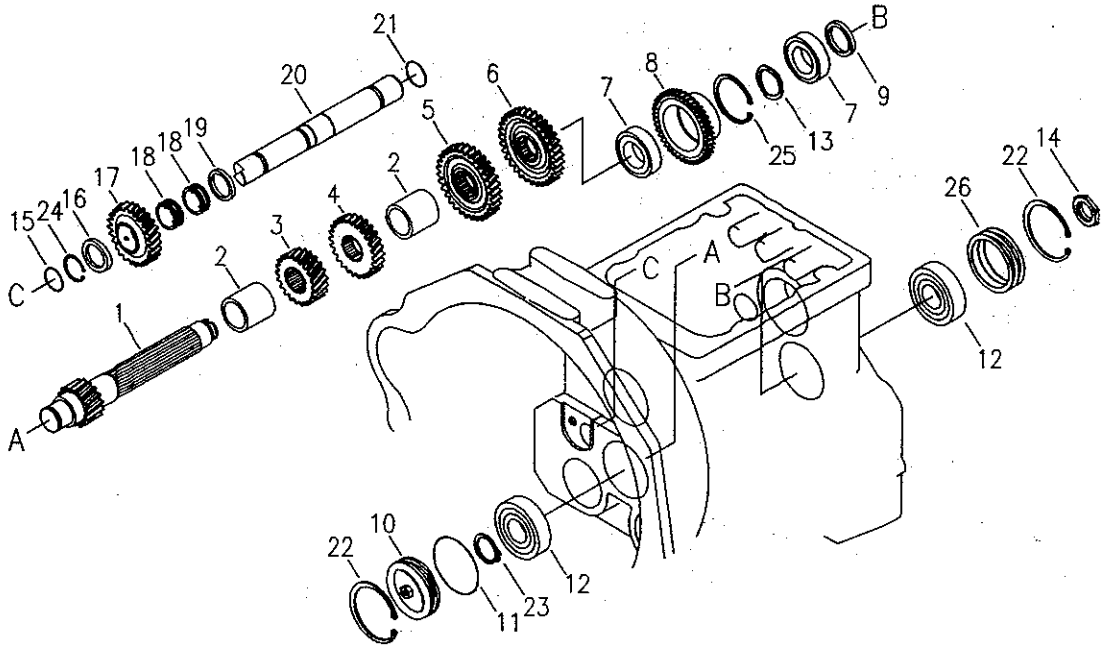
MAIN SHAFT (281)
