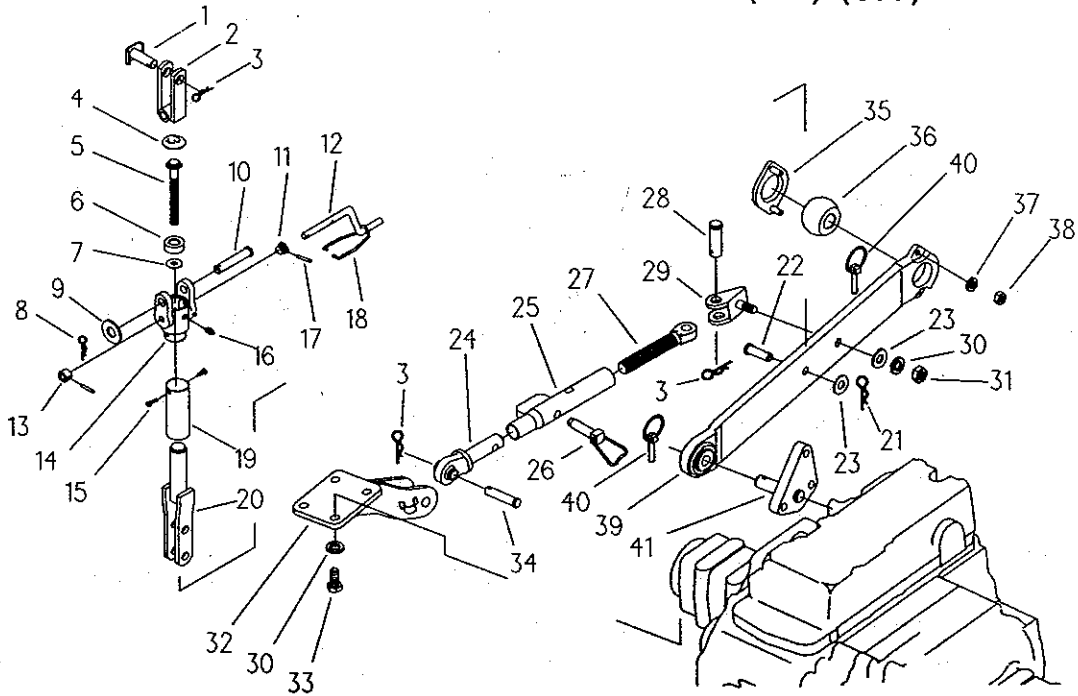
FIG 9-5 3-POINT LINKAGE-LOWER LINK(RH) (896)
