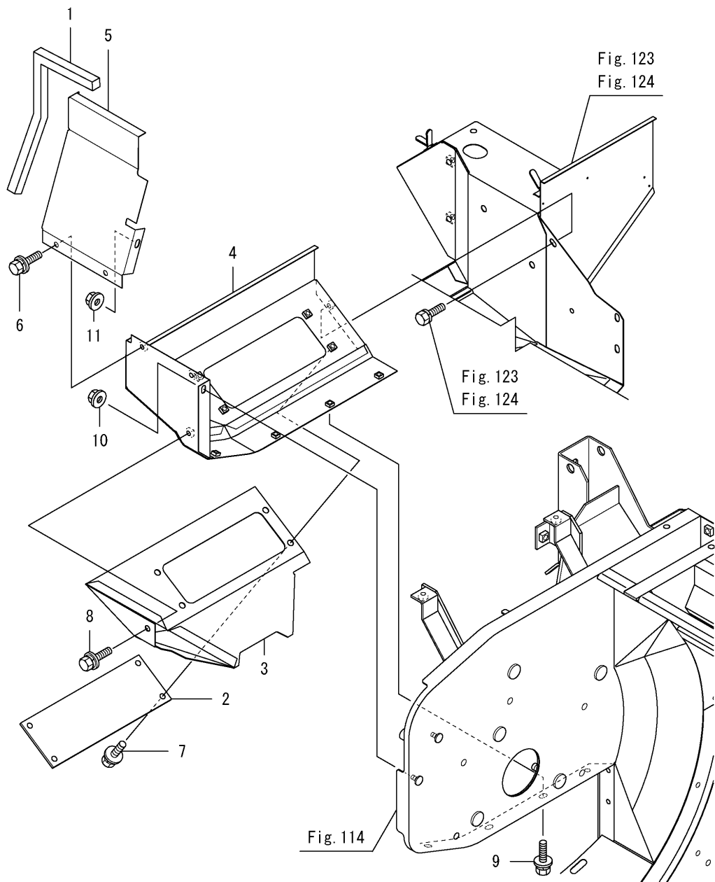
Fig.138. 탈곡통커버(앞)(1)
