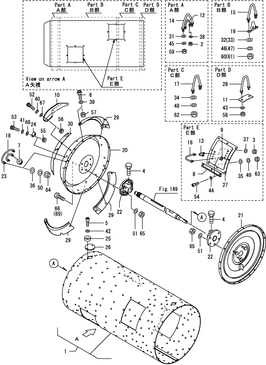
OCNP5-M34400 탈곡(1) Fig.148. 탈곡통
